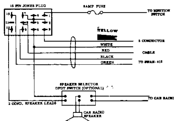
FIGURE 3 JONES PLUG WIRING DIAGRAM
