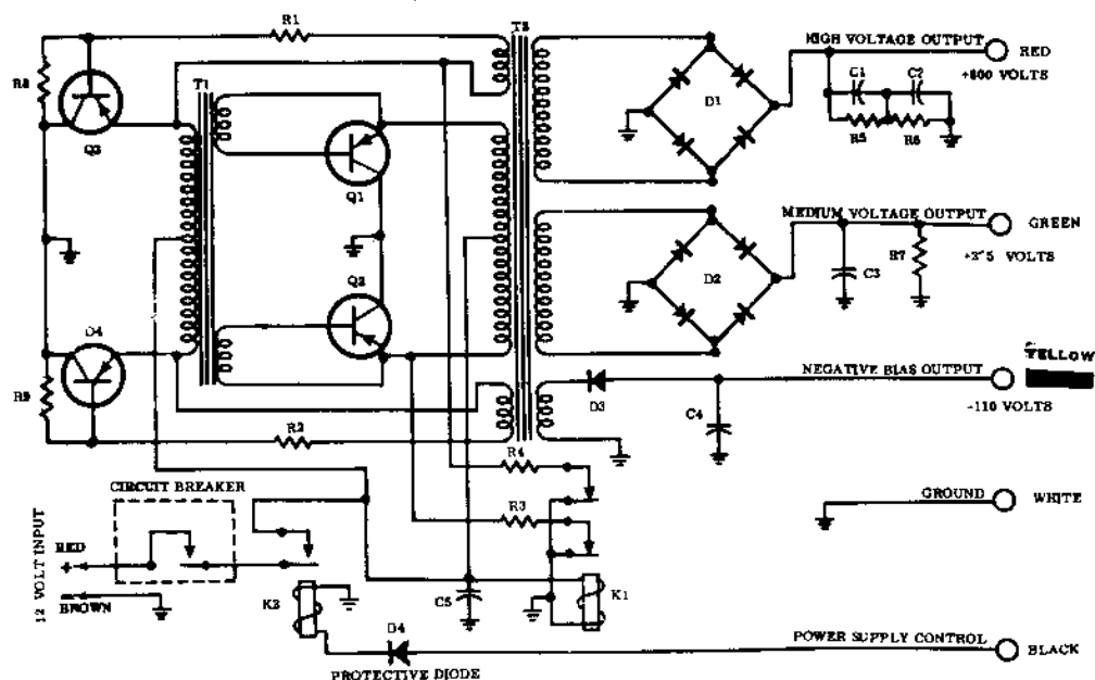
FIGURE 1 SCHEMATIC DIAGRAM, MODEL 412 DC POWER SUPPLY
