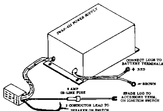
FIGURE 2 CABLING DIAGRAM
