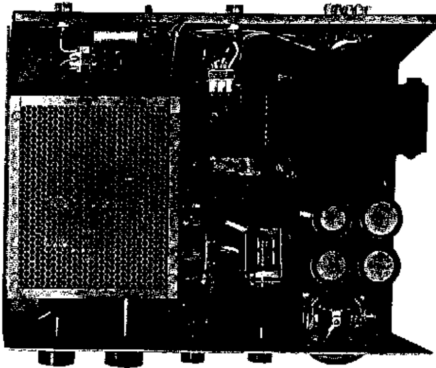
FIG. 1 - VHF-150 AMPLIFIER, TOP VIEW
