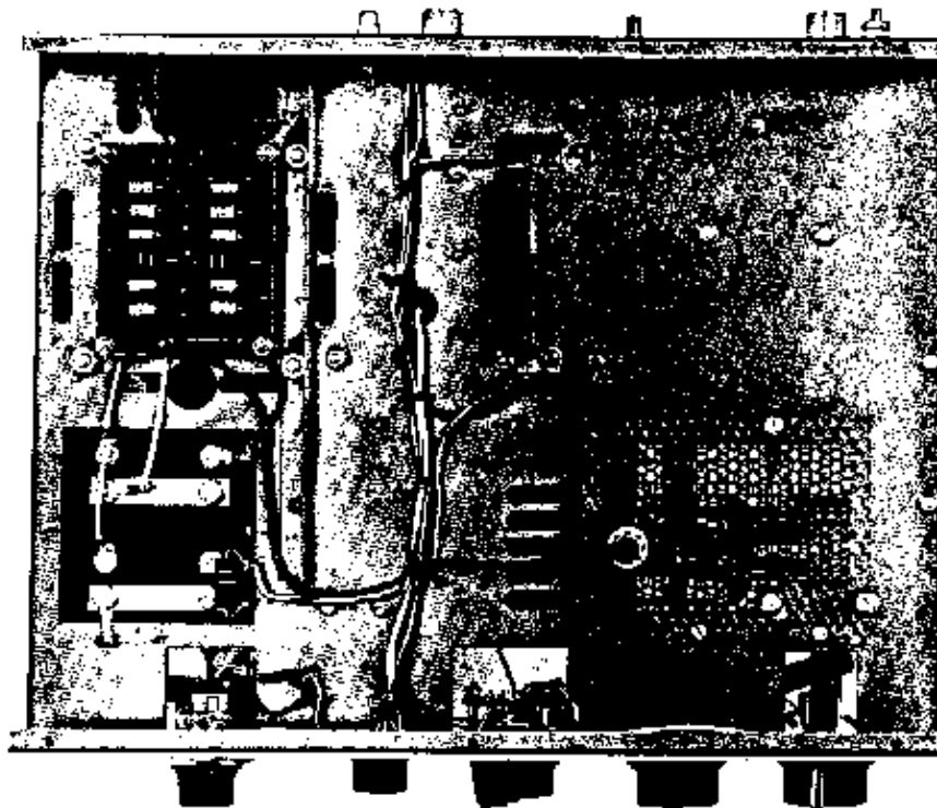
FIG. 2 - VHF-150 AMPLIFIER, BOTTOM VIEW
