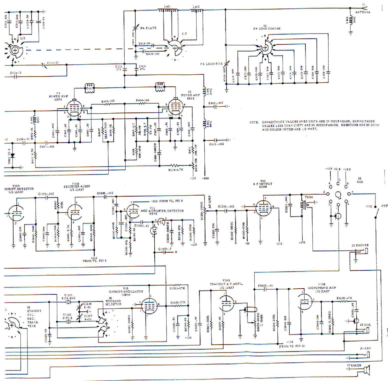
SCHEMATIC DIAGRAM, SWAN MODEL 400 SINGLE SIDEBAND TRANSCEIVER
