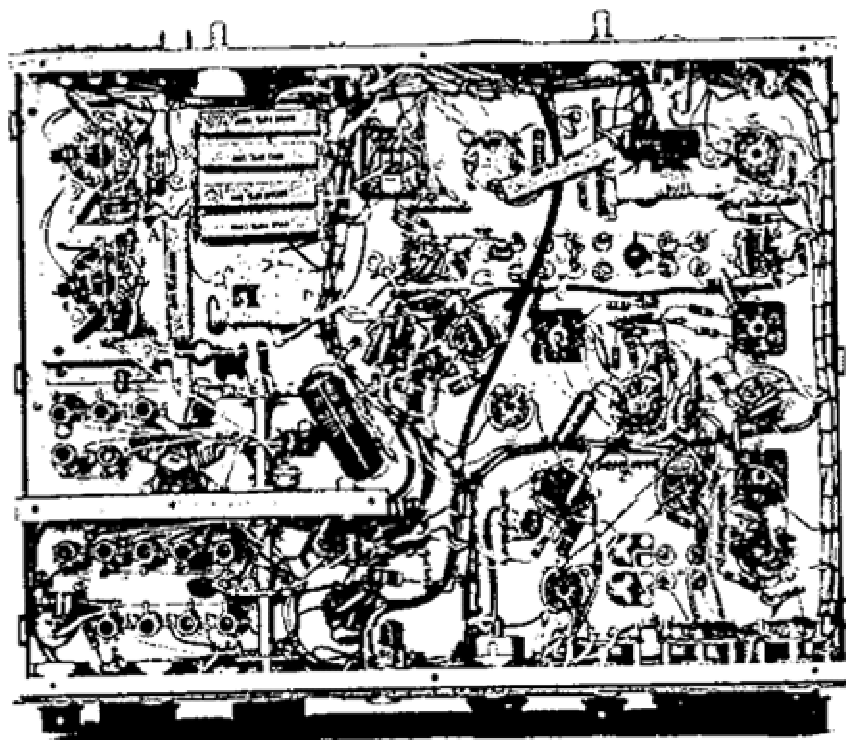
FIGURE 5 BOTTOM VIEW, MODEL 400 TRANSCIEVER
