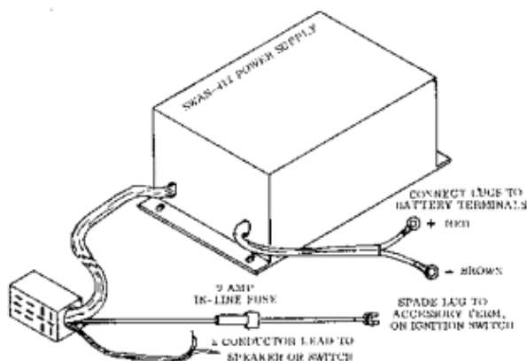
FIGURE 8 CABLING DIAGRAM
