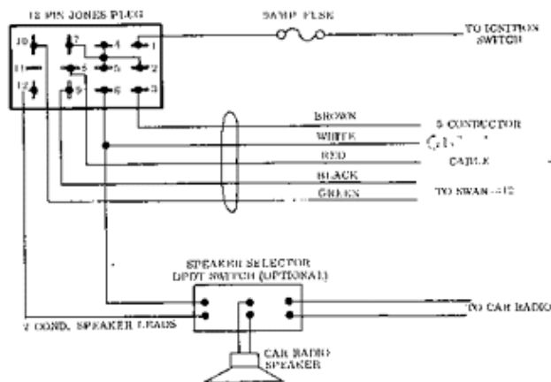
FIGURE 9 JONES PLUG WIRING DIAGRAM
