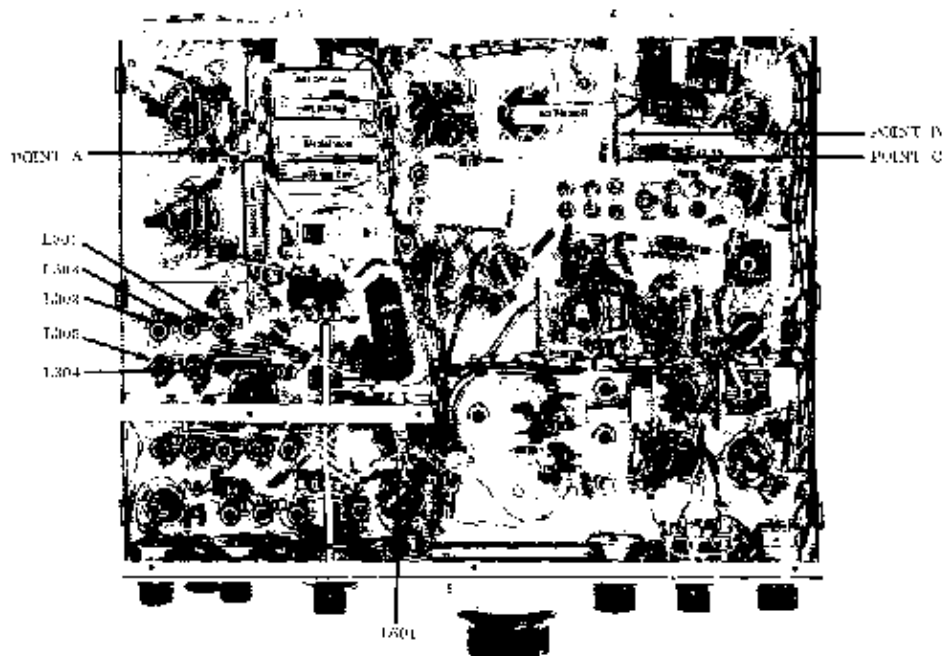
FIGURE 5 BOTTOM VIEW, MODEL 350 TRANSCIEVER
