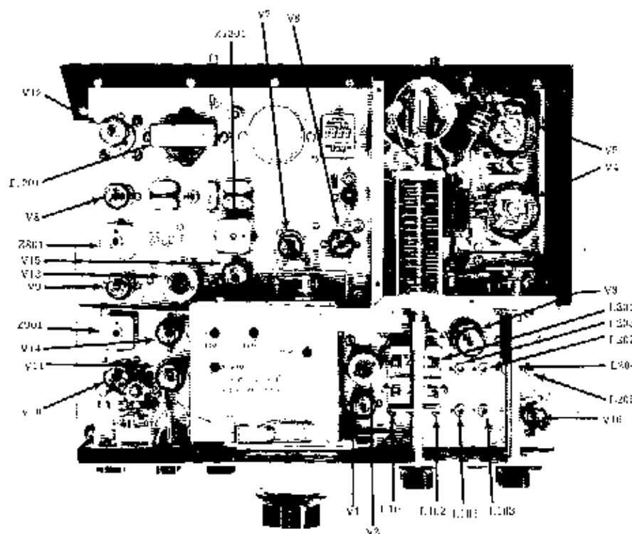
FIGURE 4 TOP VIEW, MODEL 350 TRANSCIEVER.
