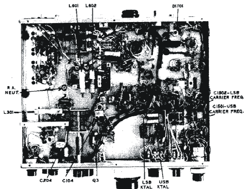
FIGURE 5 BOTTOM VIEW MODEL 250C TRANSCEIVER
