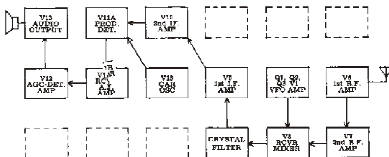
FIGURE 1 BLOCK DIAGRAM, RECEIVE MODE
