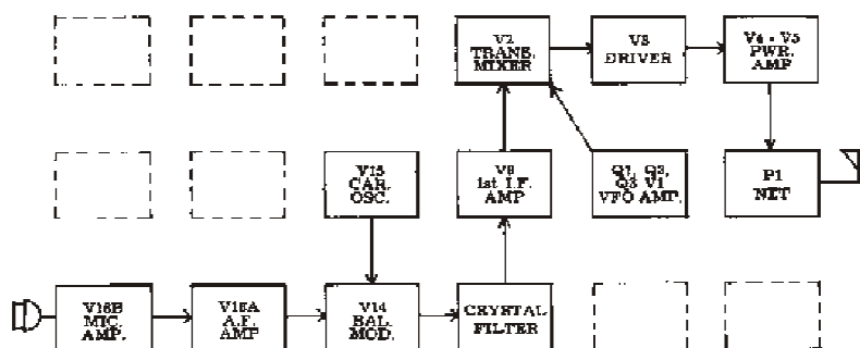
FIGURE 2 BLOCK DIAGRAM, TRANSMIT MODE
