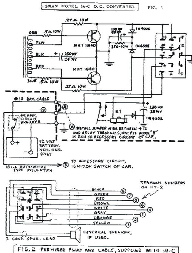
FIG. 2 PREWIRED PLUG AND CABLE, SUPPLIED WITH 14-C
