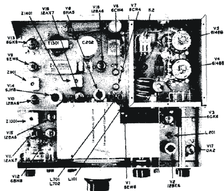
FIGURE 4 TOP VIEW MODEL 250C TRANSCEIVER
