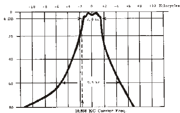
FIGURE 3 CRYSTAL FILTER, TYPICAL CHARACTERISTIC
