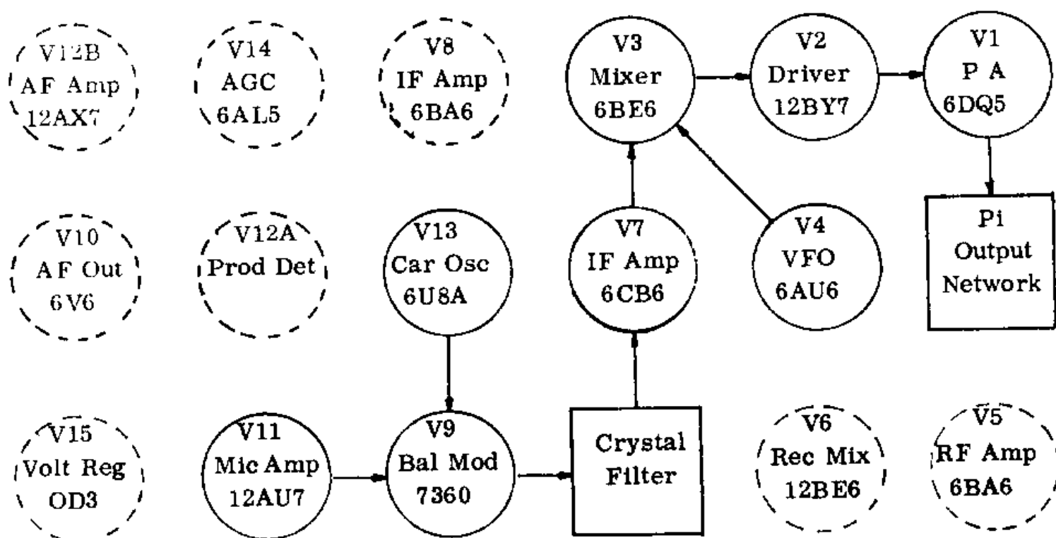
FIGURE 1. BLOCK DIAGRAM, TRANSMIT POSITION
