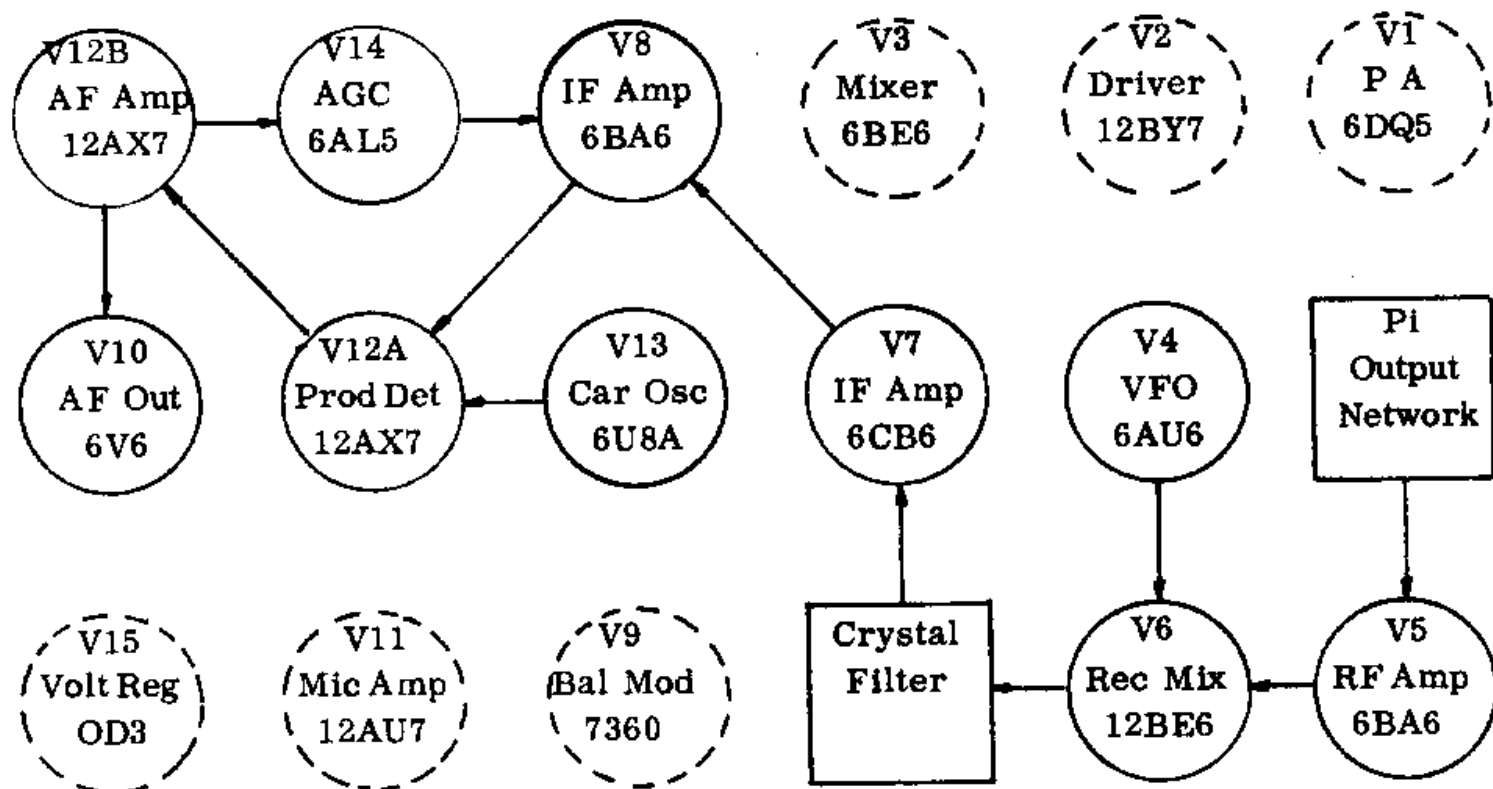
FIGURE 2. BLOCK DIAGRAM o RECEIVE POSITION
