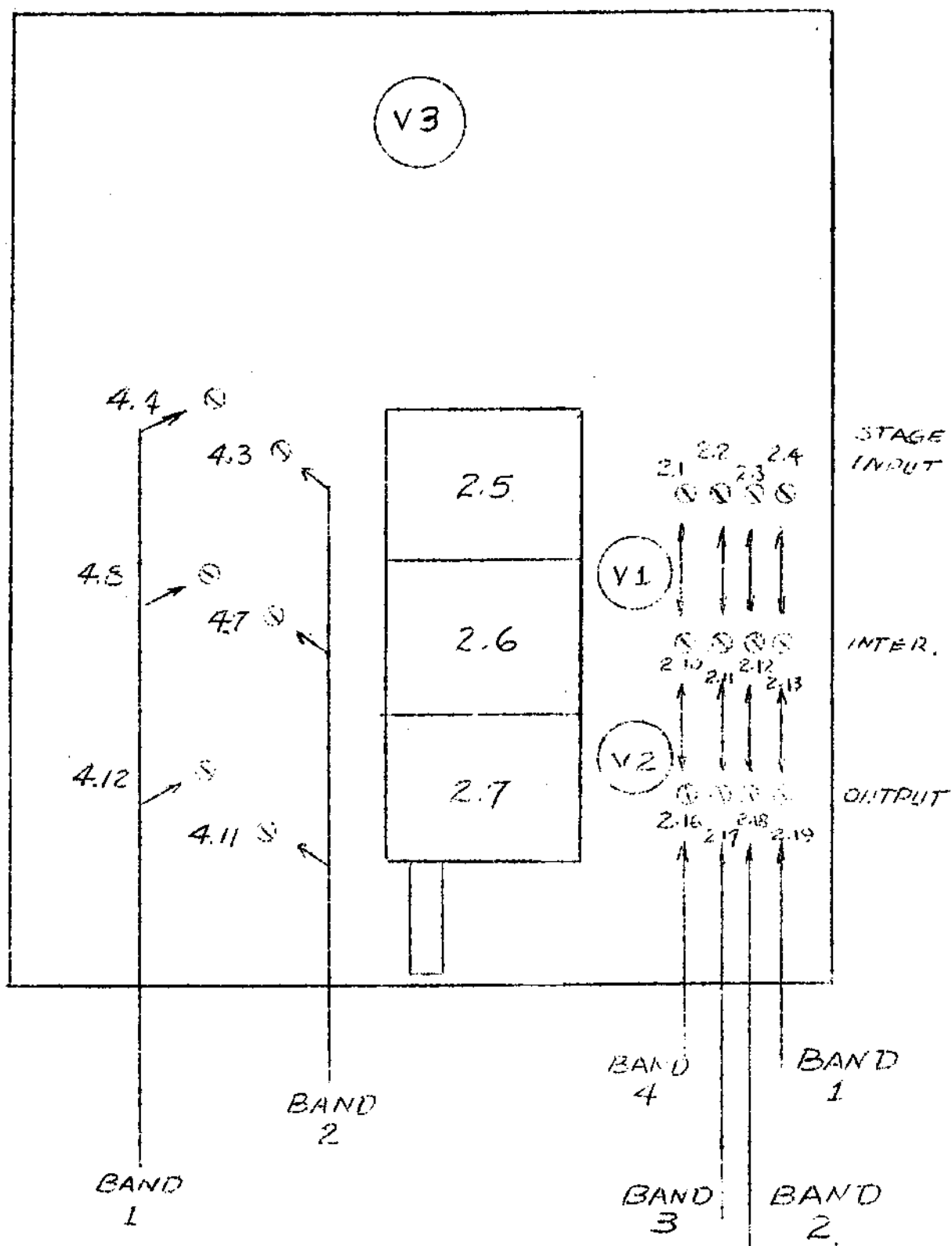
TOP VIEW OF CHASSIS
