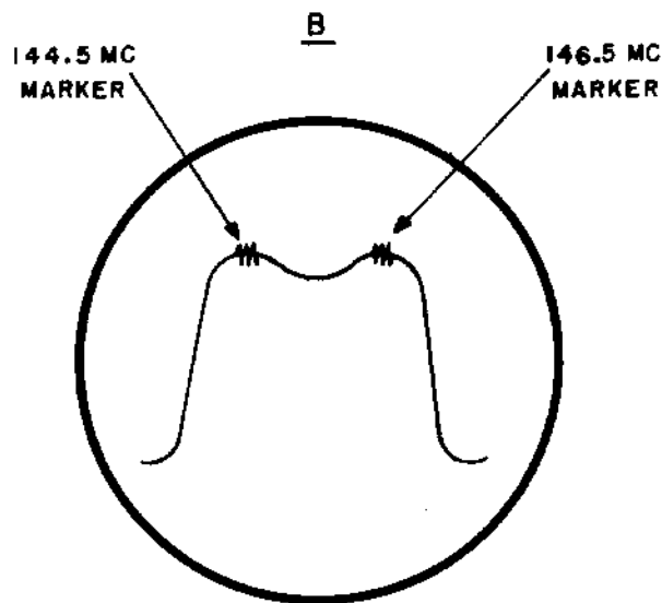
Figure 5. NC-300C2, Rectifier-Filter Network and Scope Pattern
