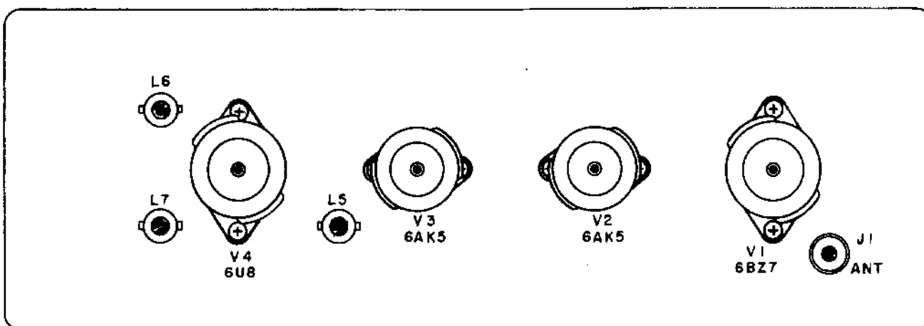
Figure 4. NC-300C2, Top View
