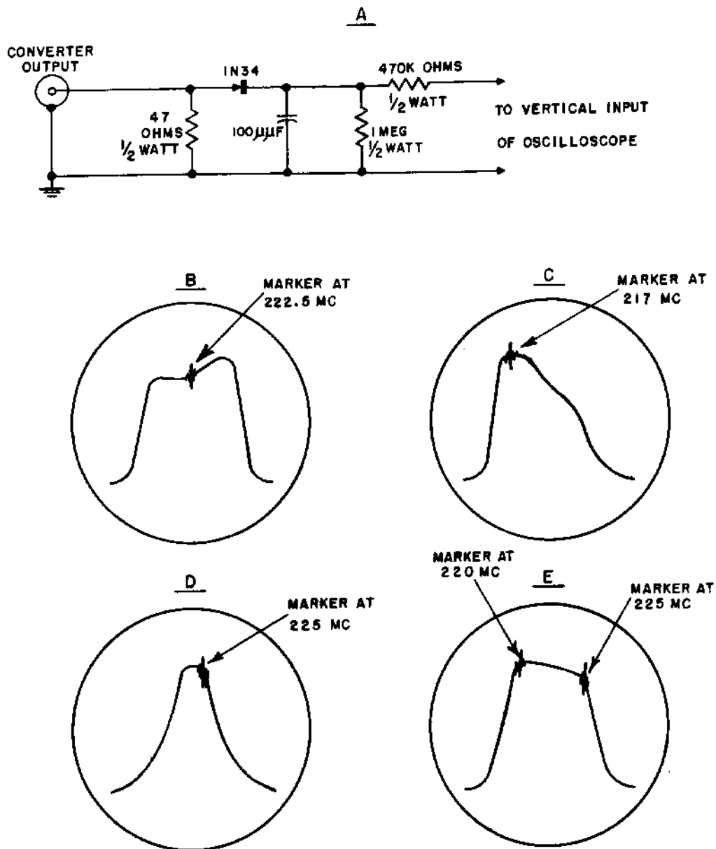
Figure 8. NC-300C1, Rectifier-Filter Network and Scope Patterns
