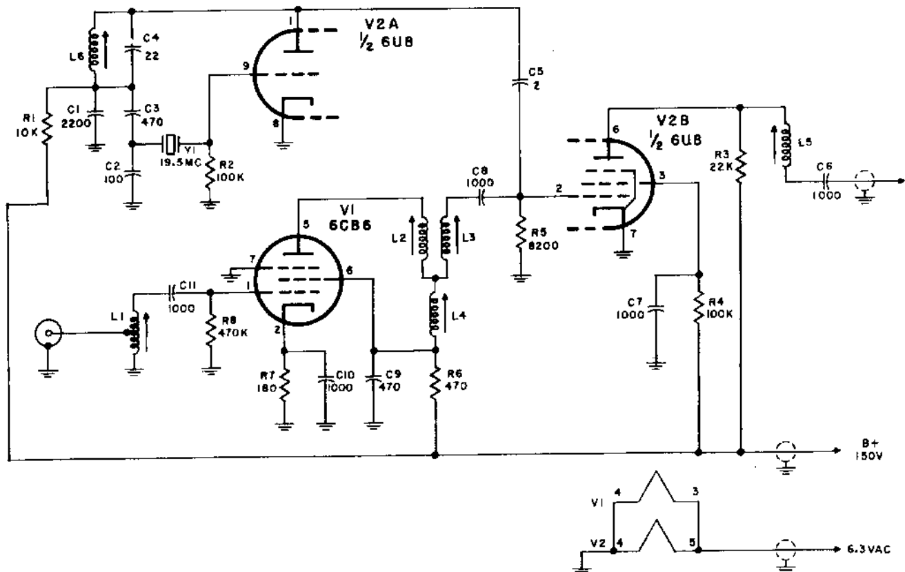
Figure 3. NC-300C6A, Schematic Diagram
