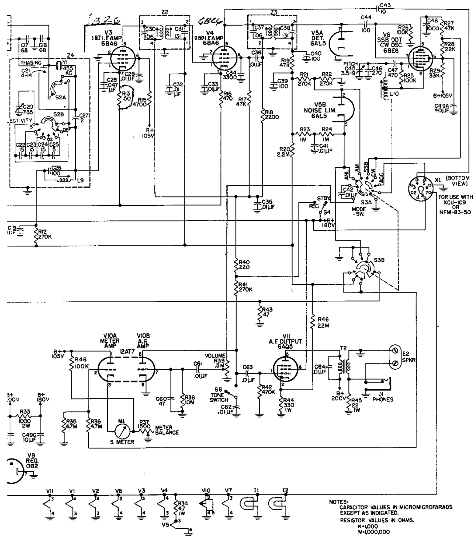
NC109 Receiver Schematic Diagram
