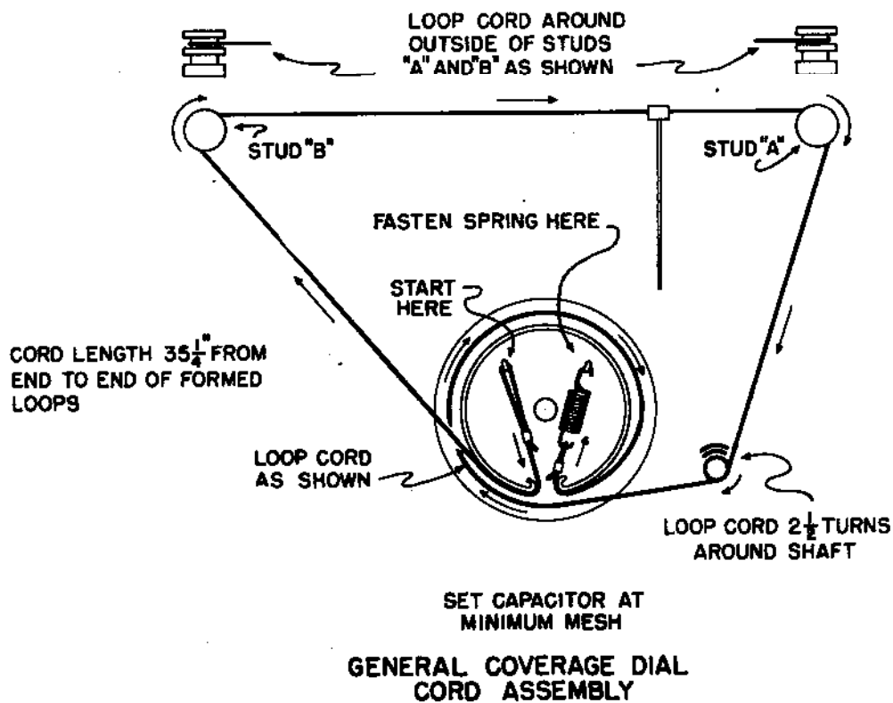
Figure 4-1. Dial Stringing Diagrams
