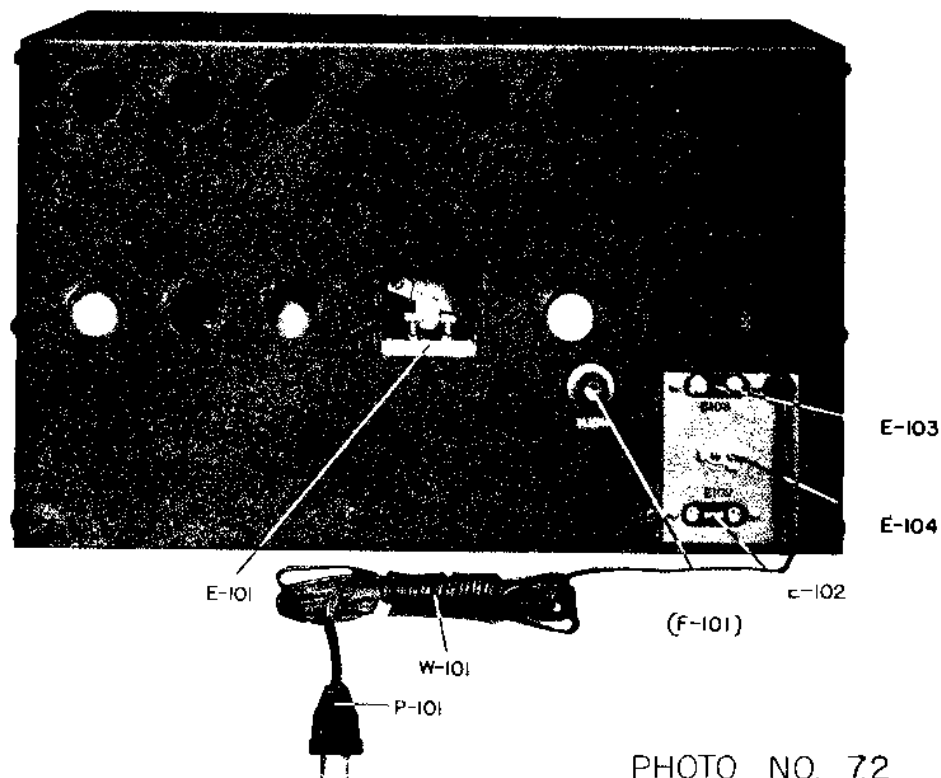
REAR VIEW OF RECEIVER
