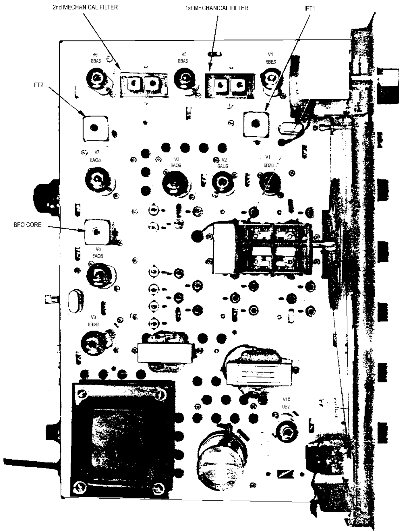
FIGURE 6. ALIGNMENT POINTS (TOP VIEW)
