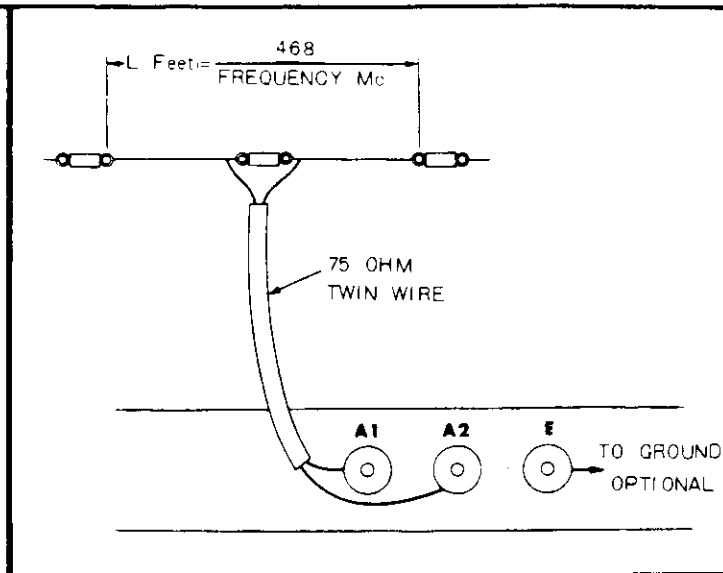
Figure 2. Doublet Antenna
