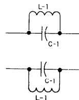
50 mc TRAP
