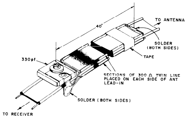
1/4-WAVE TRAP
