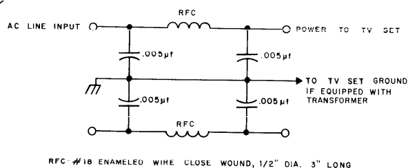
AC POWER LINE FILTER
