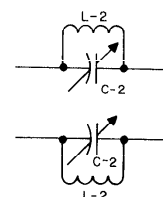
144 mc TRAP
