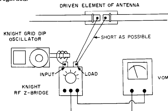
FIGURE 12. COUPLING TO AN ANTENNA THROUGH AN SWR BRIDGE.
