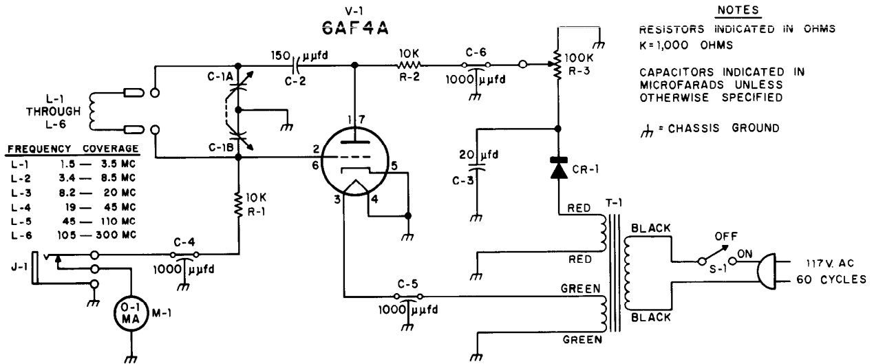
SCHEMATIC DIAGRAM OF GRID DIP METER
