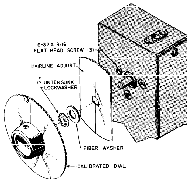
FIGURE 8. MOUNTING THE DIAL
