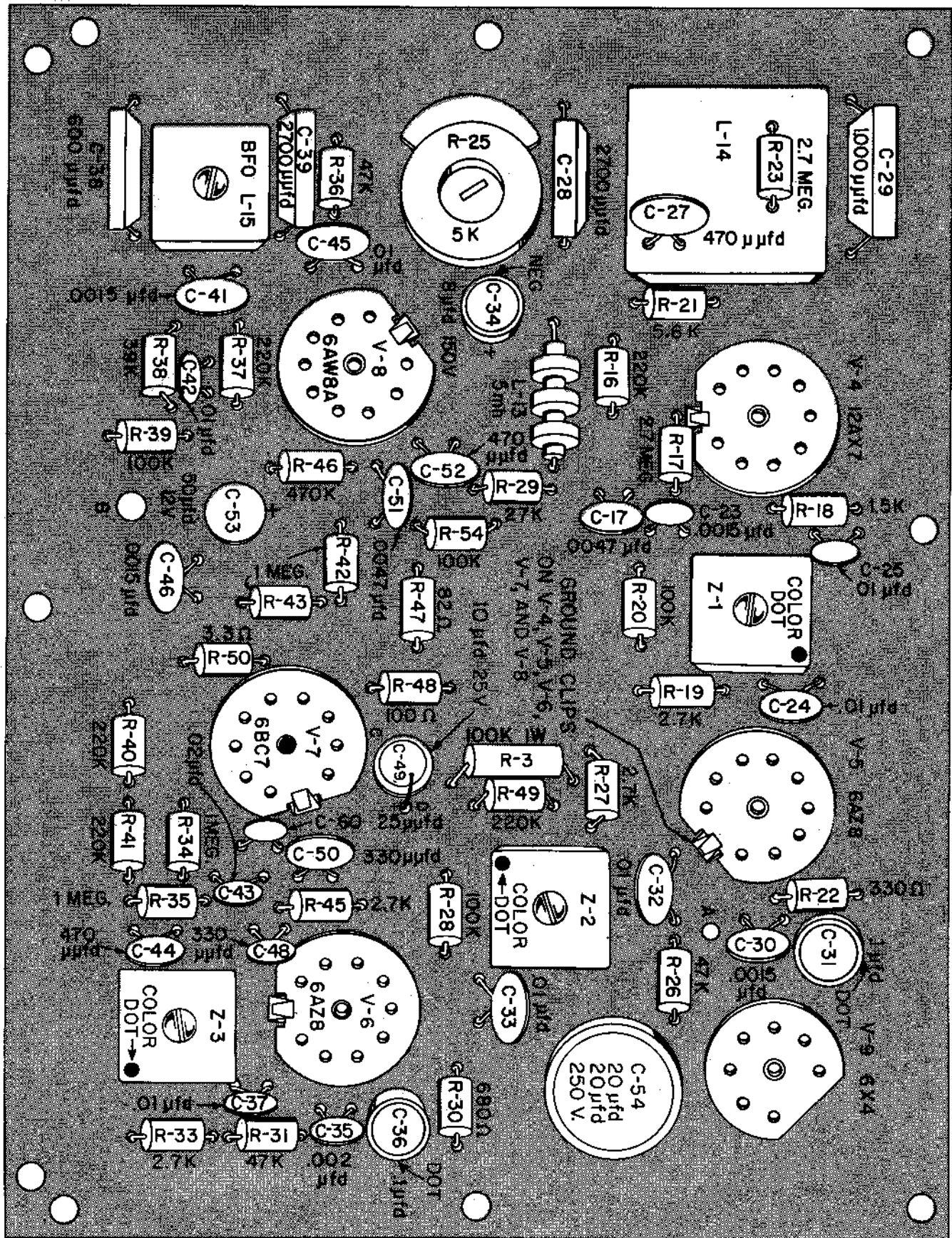
FIGURE 1. PARTS MOUNTING ON THE IF PRINTED CIRCUIT BOARD
