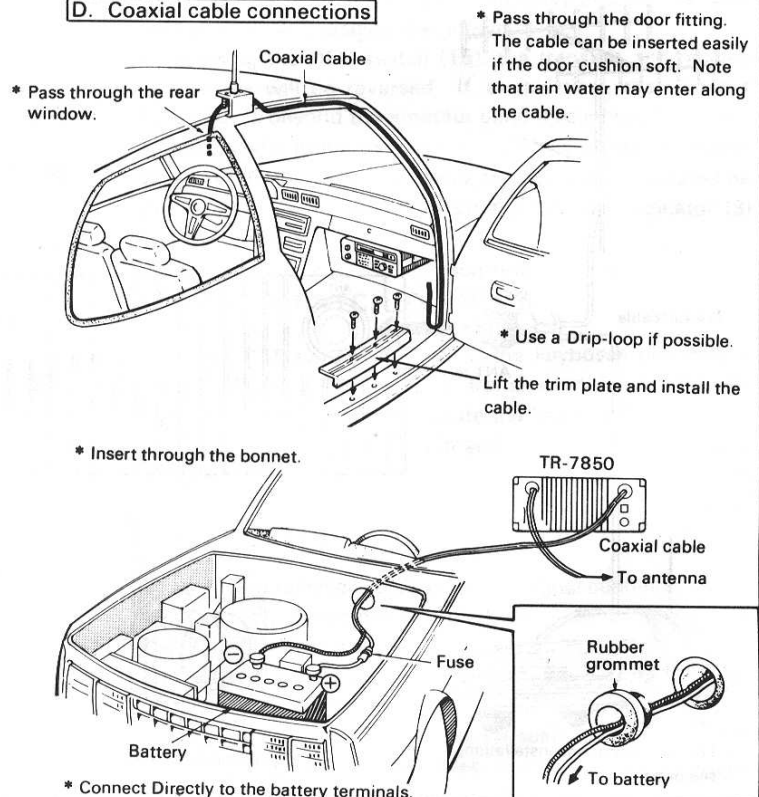
Fig. 1-2 Installation for Mobile Operation
