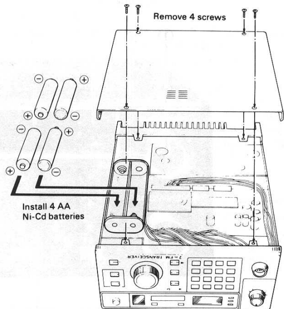
Fig. 1-4 Battery Back-up
