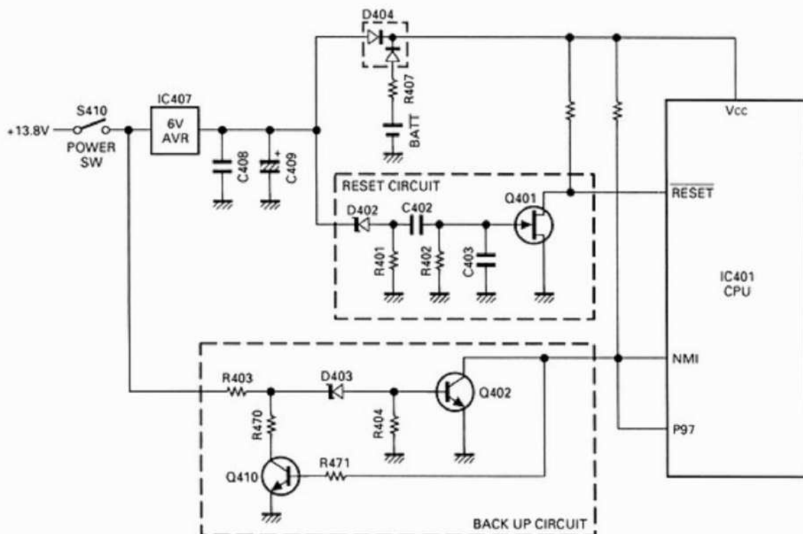
Fig. 18 Reset and backup circuits
