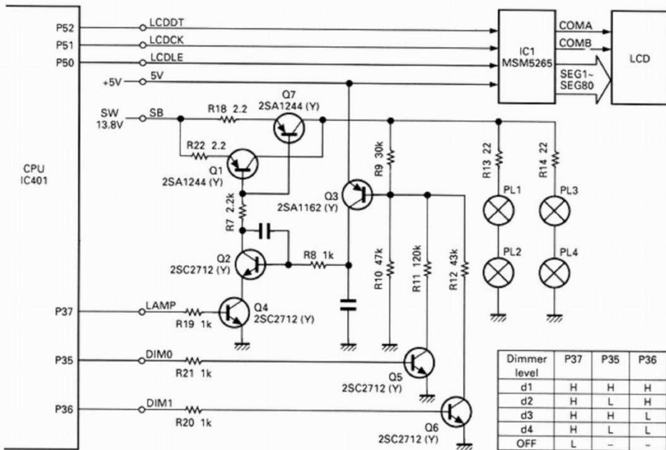
Fig. 19 Display and dimmer circuits
