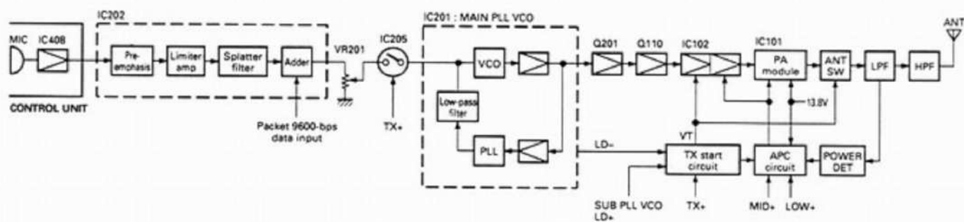
Fig. 5 Transmitter system block diagram
