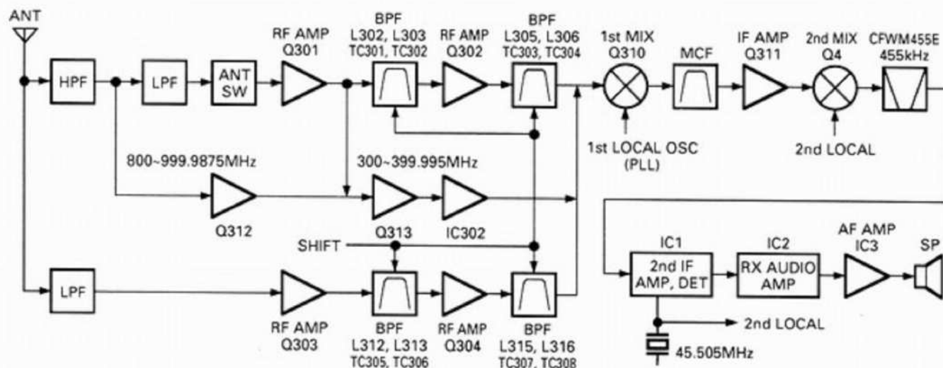
Fig. 2 Receiver system configuration
