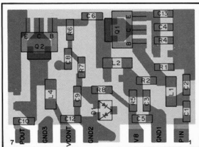
IC102 : RF AMP (W02-1831-08) Foil side view
