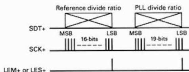
Fig. 20 Data transfer format
