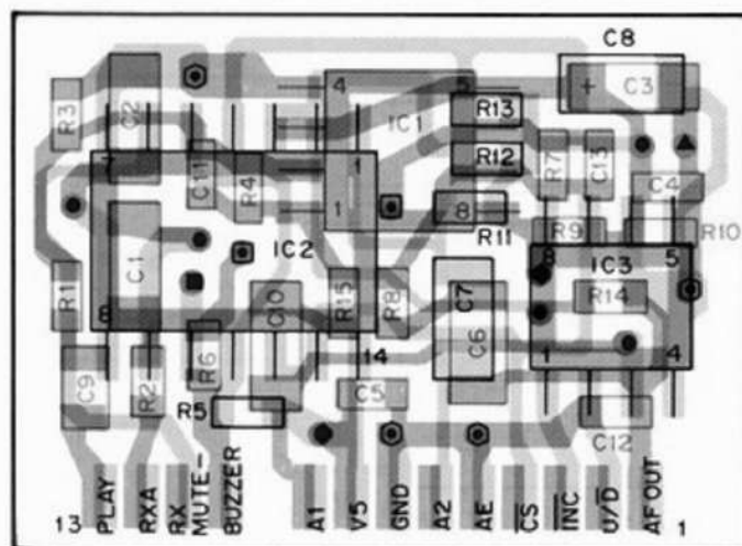
IC2 : RX AUDIO (W02-1829-08) Component side view
