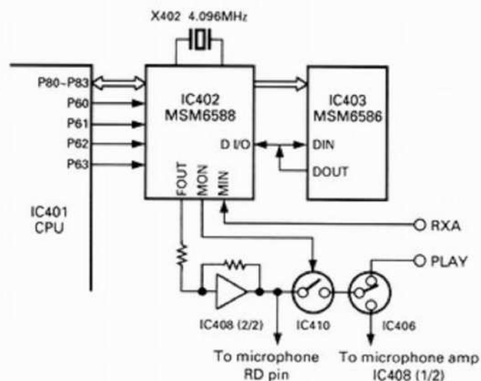
Fig. 24 Digital recording circuit
