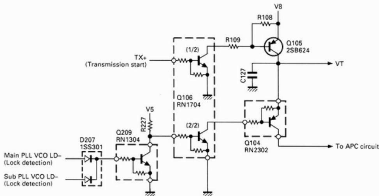
Fig. 12 Transmission start circuit
