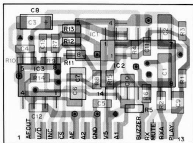
IC2 : RX AUDIO (W02-1829-08) Foil side view
