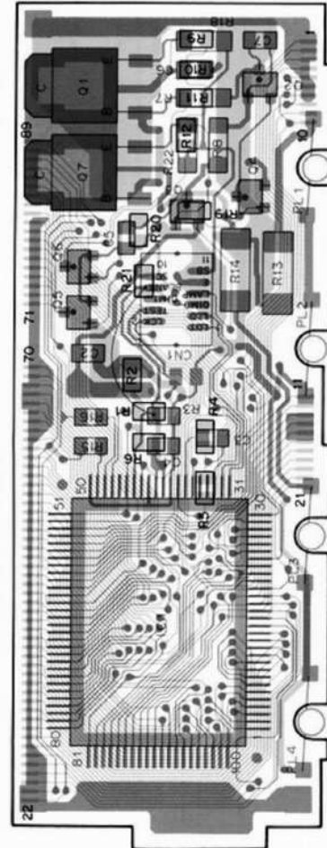
LCD ASSY (B38-0721-08) Foil side view
