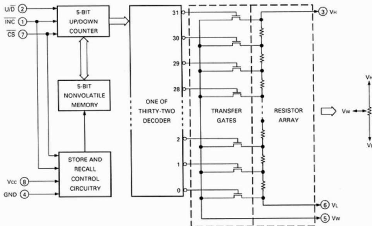
Fig. 14 Electronic VR (X9313) block diagram
