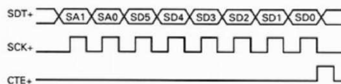
Fig. 25 Data transfer format
