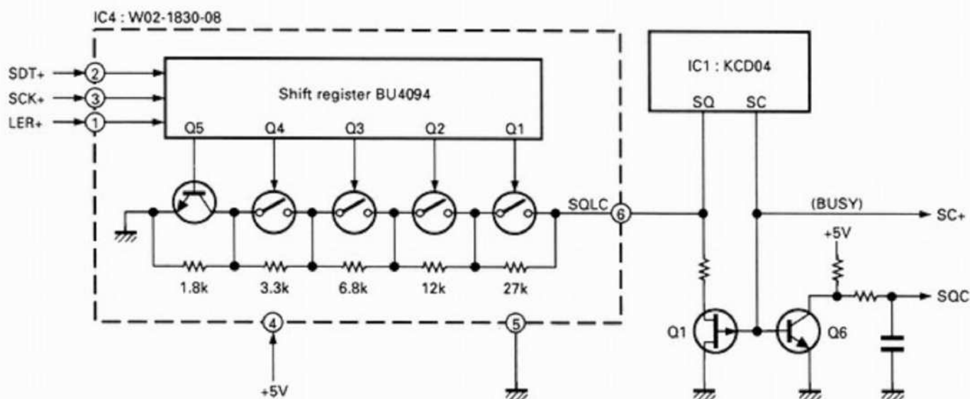
Fig. 15 Squelch circuit
