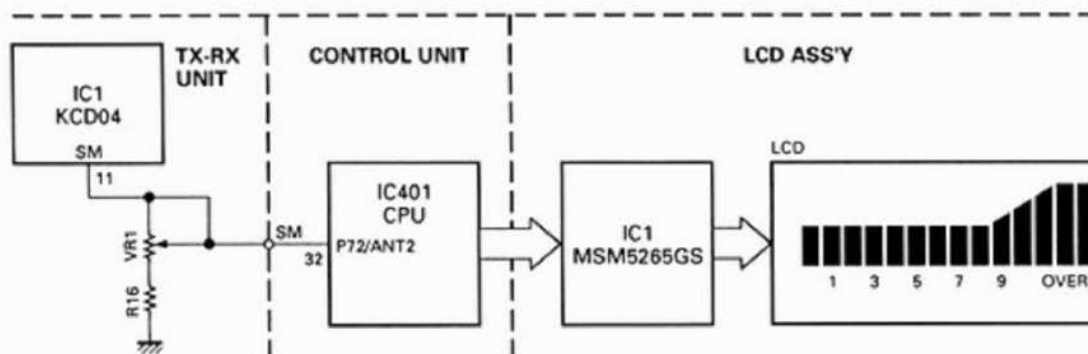
Fig. 3 S-meter circuit
