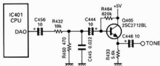
Fig. 22 Tone output circuit
