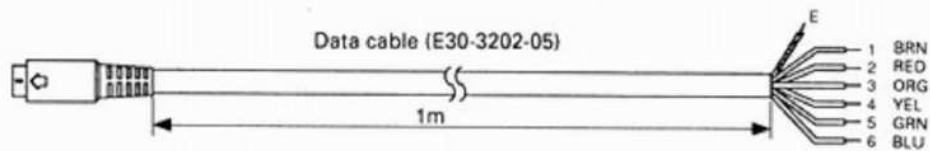
PG-5A Dimension
