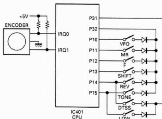
Fig. 16 Key and rotary encoder input circuits
