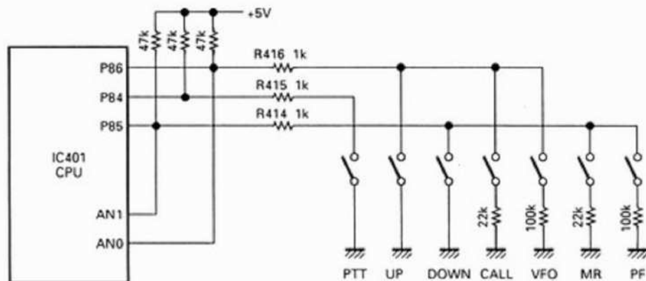
Fig. 17 Microphone key input circuit
