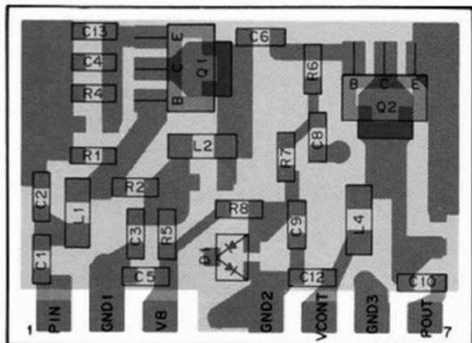
IC102 : RF AMP (W02-1831-08) Component side view
