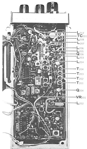
TRANSMITTER SECTION ALIGNMENT POINTS
