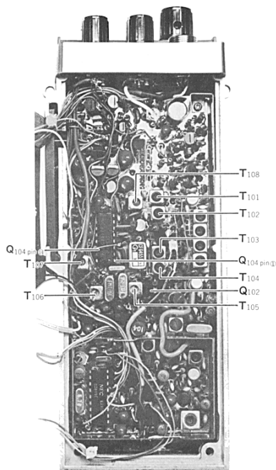
RECEIVER SECTION ALIGNMENT POINTS
