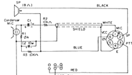
YM-24 Speaker/Microphone Connections
