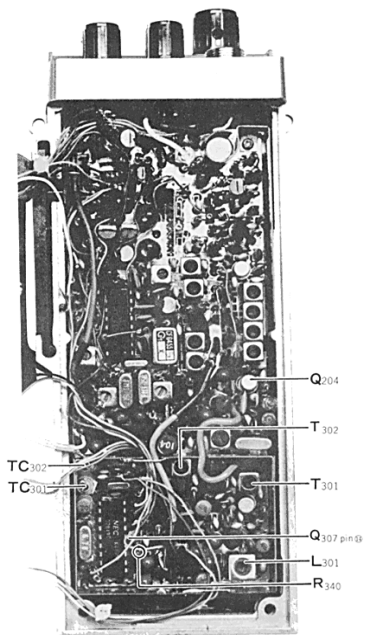
PLL SECTION ALIGNMENT POINTS
