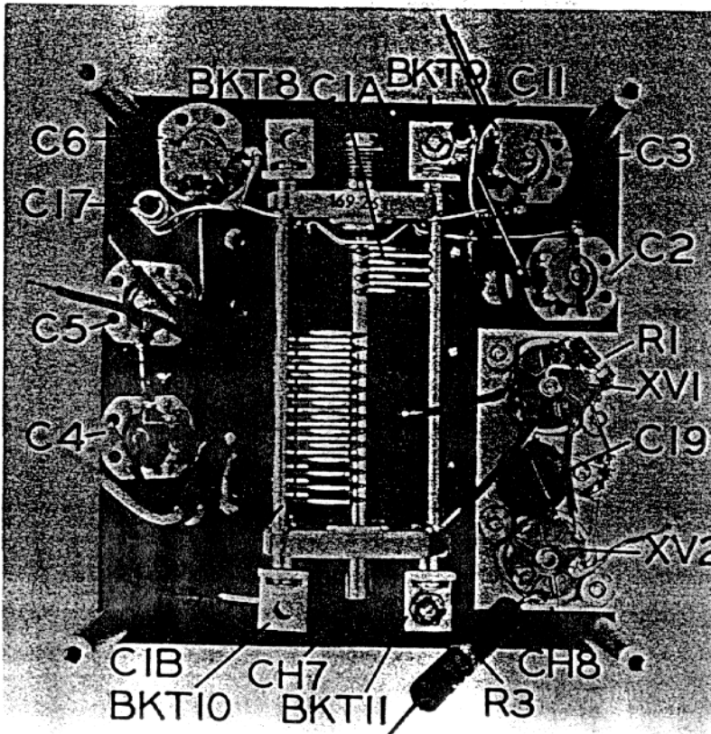
Figure 6b, VFO Chassis, Bottom View
