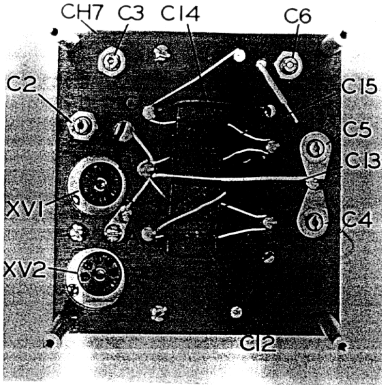
Figure 6a, VFO Chassis, Top View
