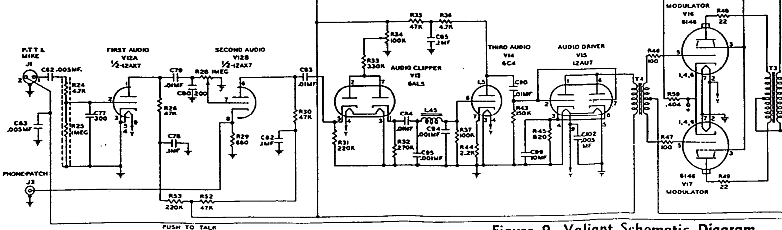
Figure 9, Valiant Schematic Diagram
