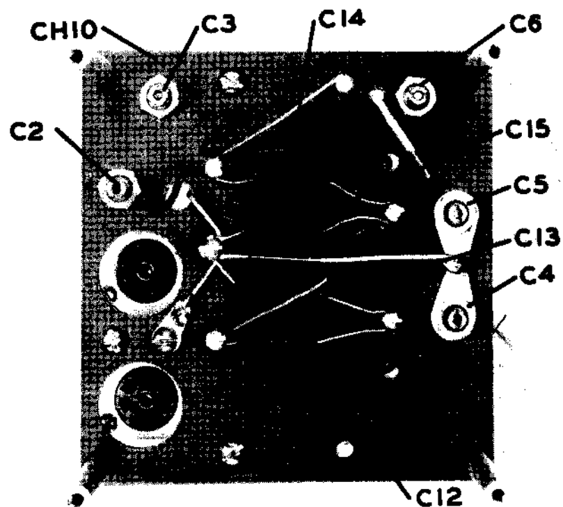
FIGURE 3A. V.F.O. CHASSIS TOP VIEW.
