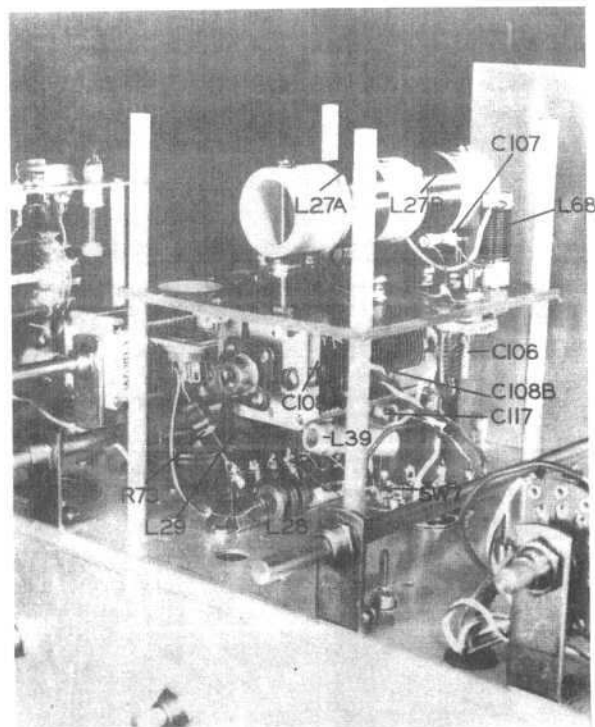
Figure 5b: VFO, Right Side
