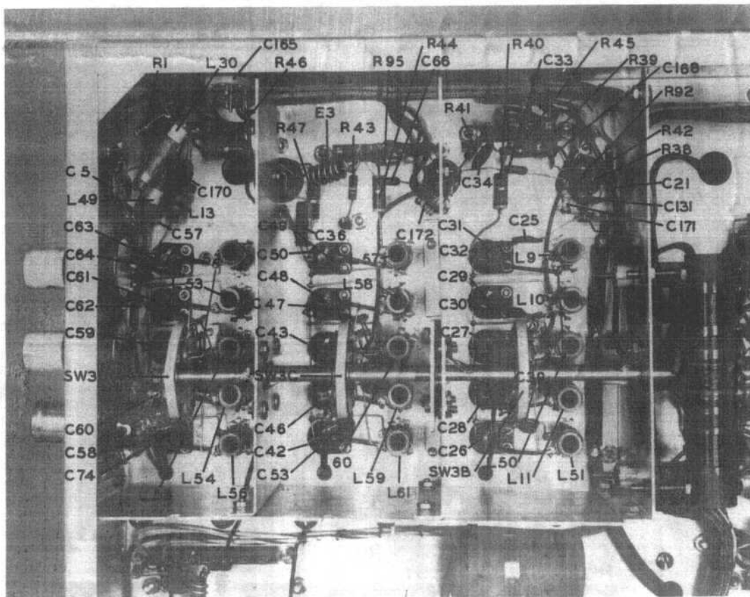
Figure 7c: RF Exciter, Bottom View
