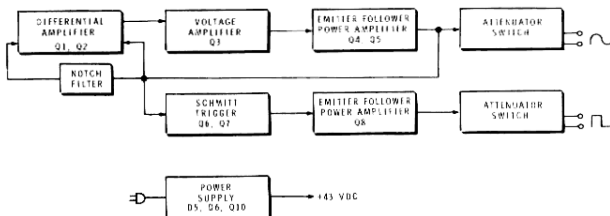
BLOCK DIAGRAM
