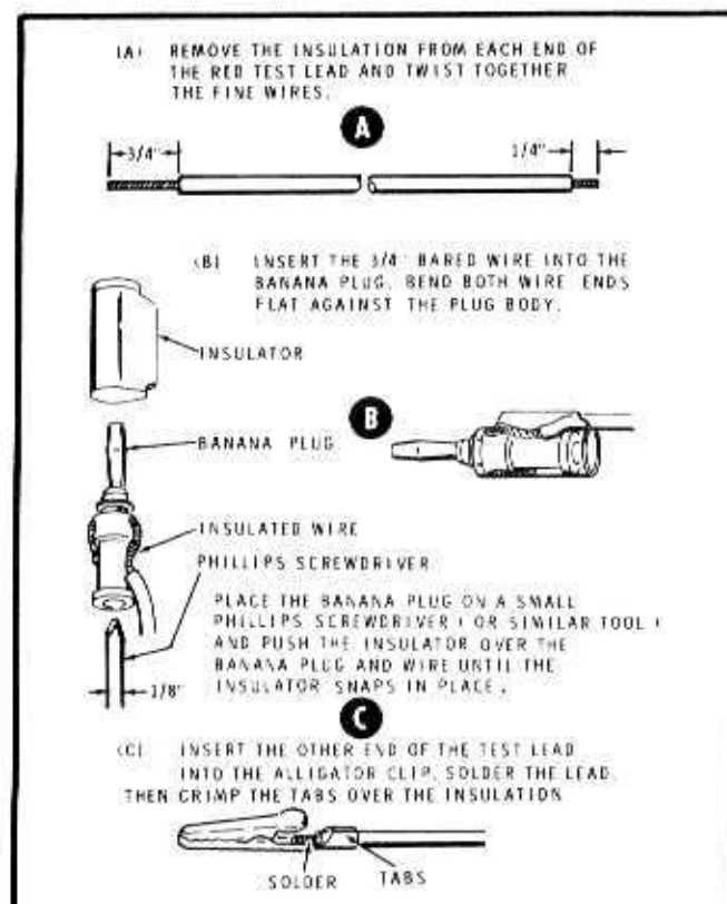
PICTORIAL 20
