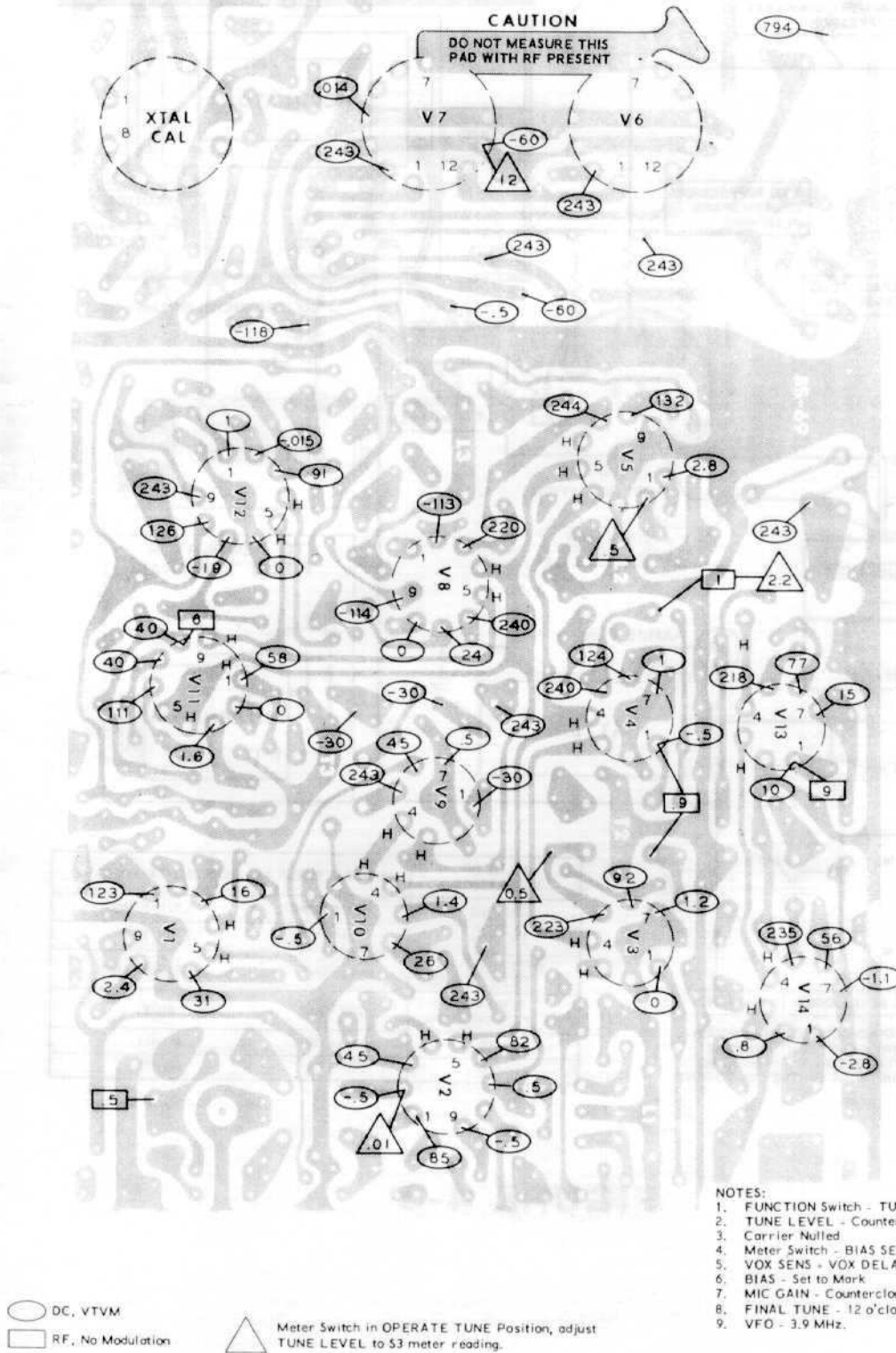
TRANSMITTER VOLTAGE CHART FIGURE 6-3
