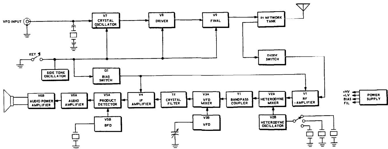
BLOCK DIAGRAM
