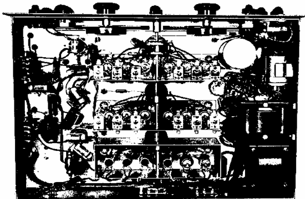
Fig. 7—Bottom view showing placement of parts.
