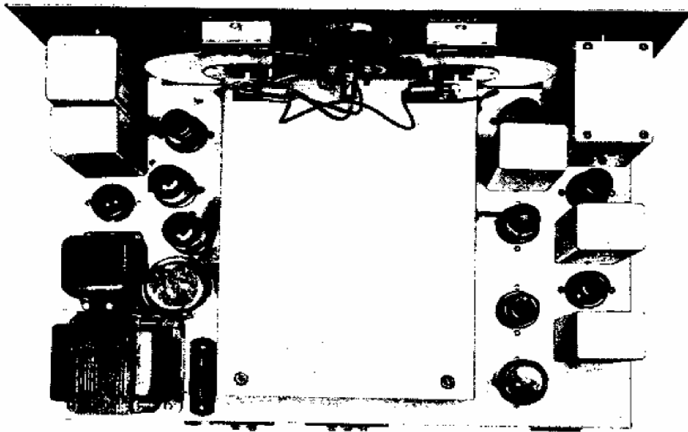
Fig. 6—Top view showing chassis layout.
