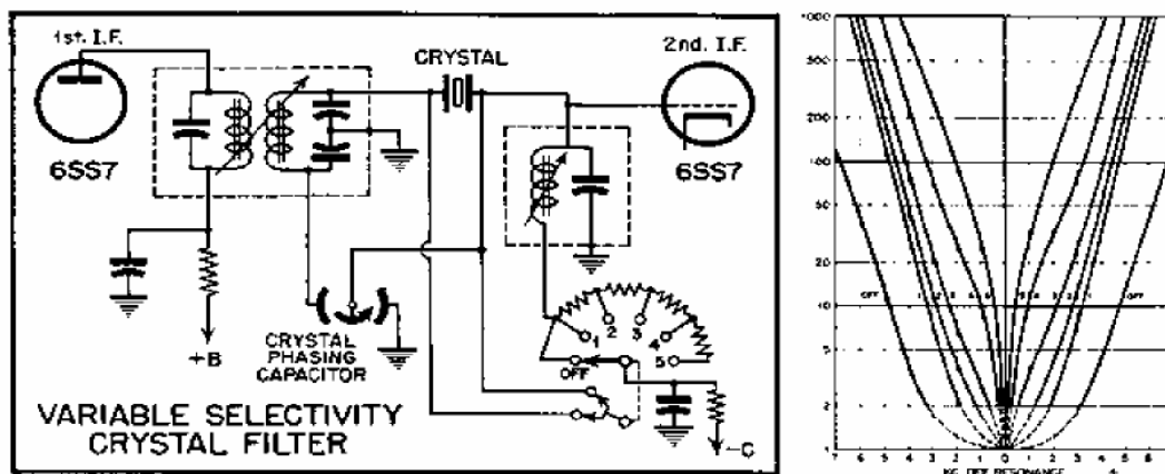
Fig. 5 Selectivity curve and crystal filter circuit.
