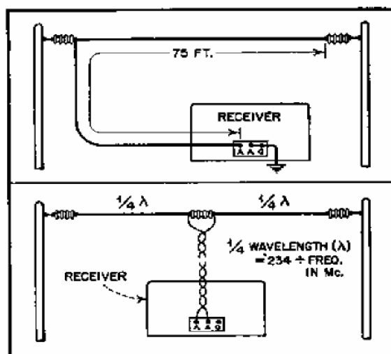
Fig. 9—Antenna suggestions.
