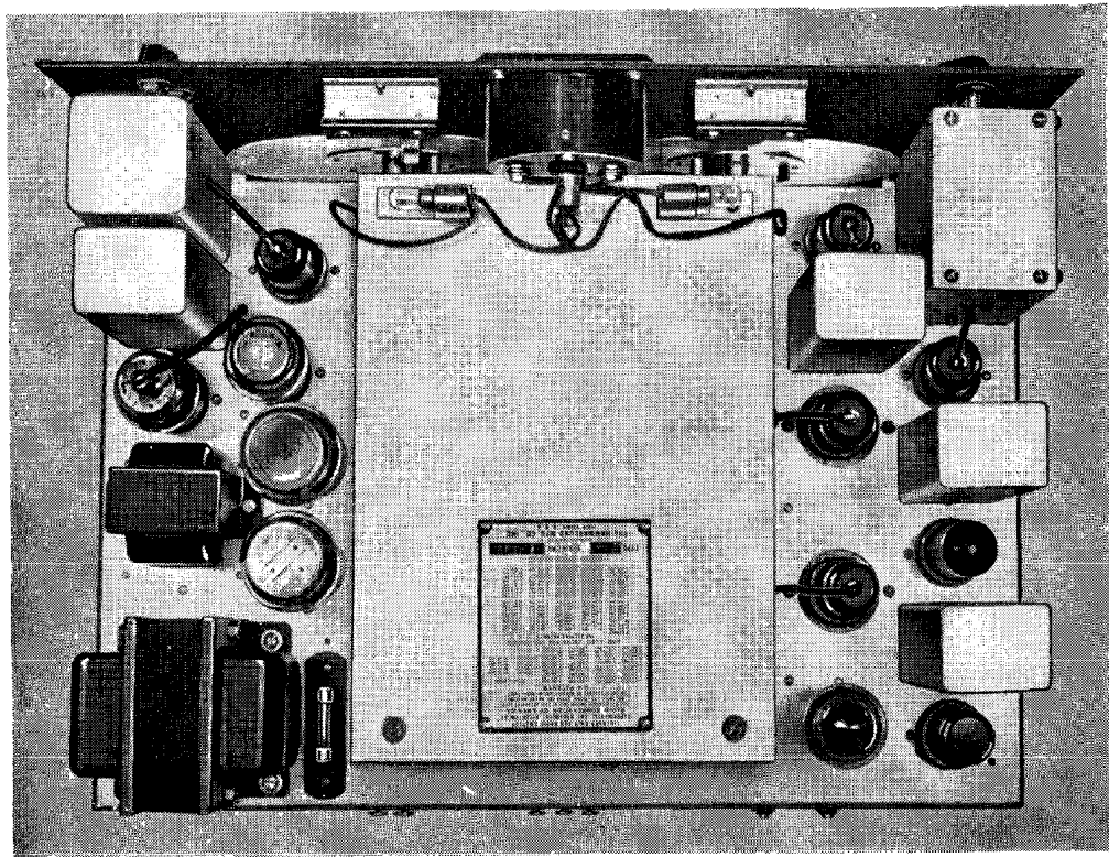
FIG. 6—Top view of "HQ-120-X," chassis.
