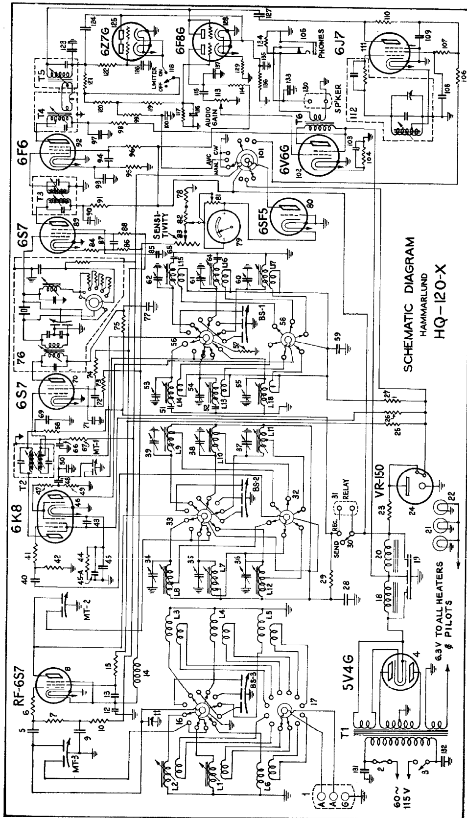
FIG. 5—Complete circuit diagram of "HQ-120-X"
