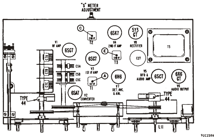
Fig. 7. Top View of Chassis Showing Tube Locations and Alignment Adjustments
