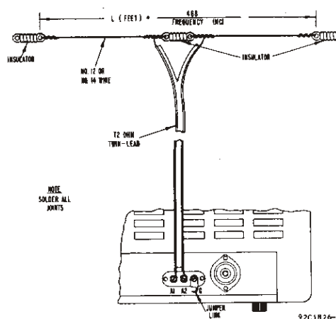
Fig. 3. Doublet Antenna Using Twin-Lead Lead-In
