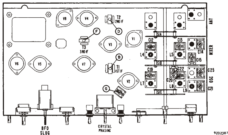
Fig. 8. Bottom View of Chassis Showing Tube Locations and Alignment Adjustments
