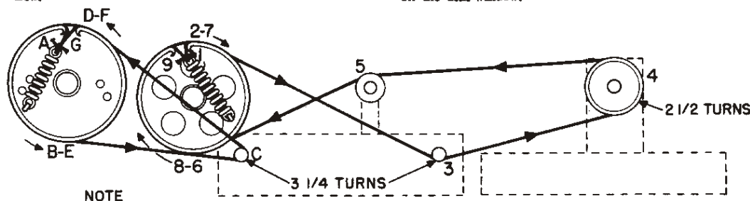
Fig. 6. Dial Cord Stringing Diagram
