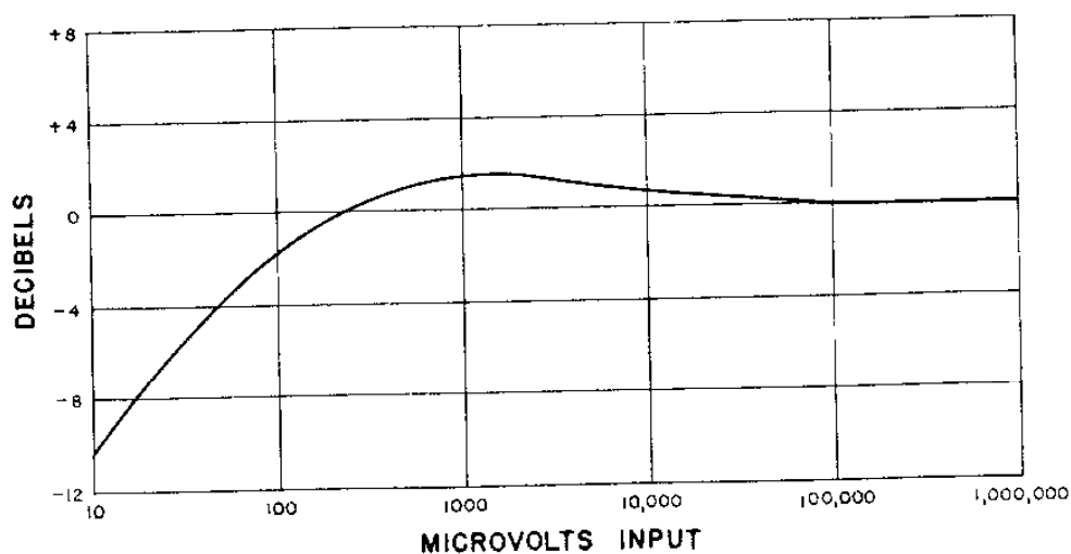
FIG. 7—A.V.C. CURVE—AT 3 MC.
