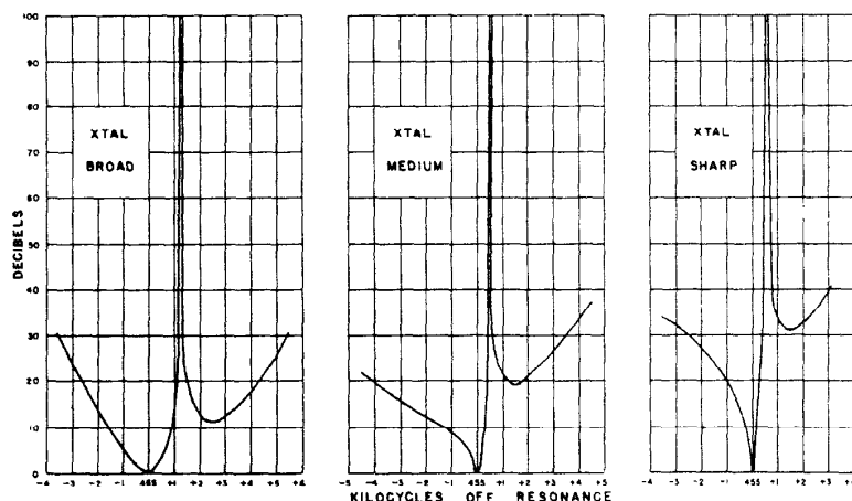
FIG. 4—CRYSTAL SELECTIVITY
