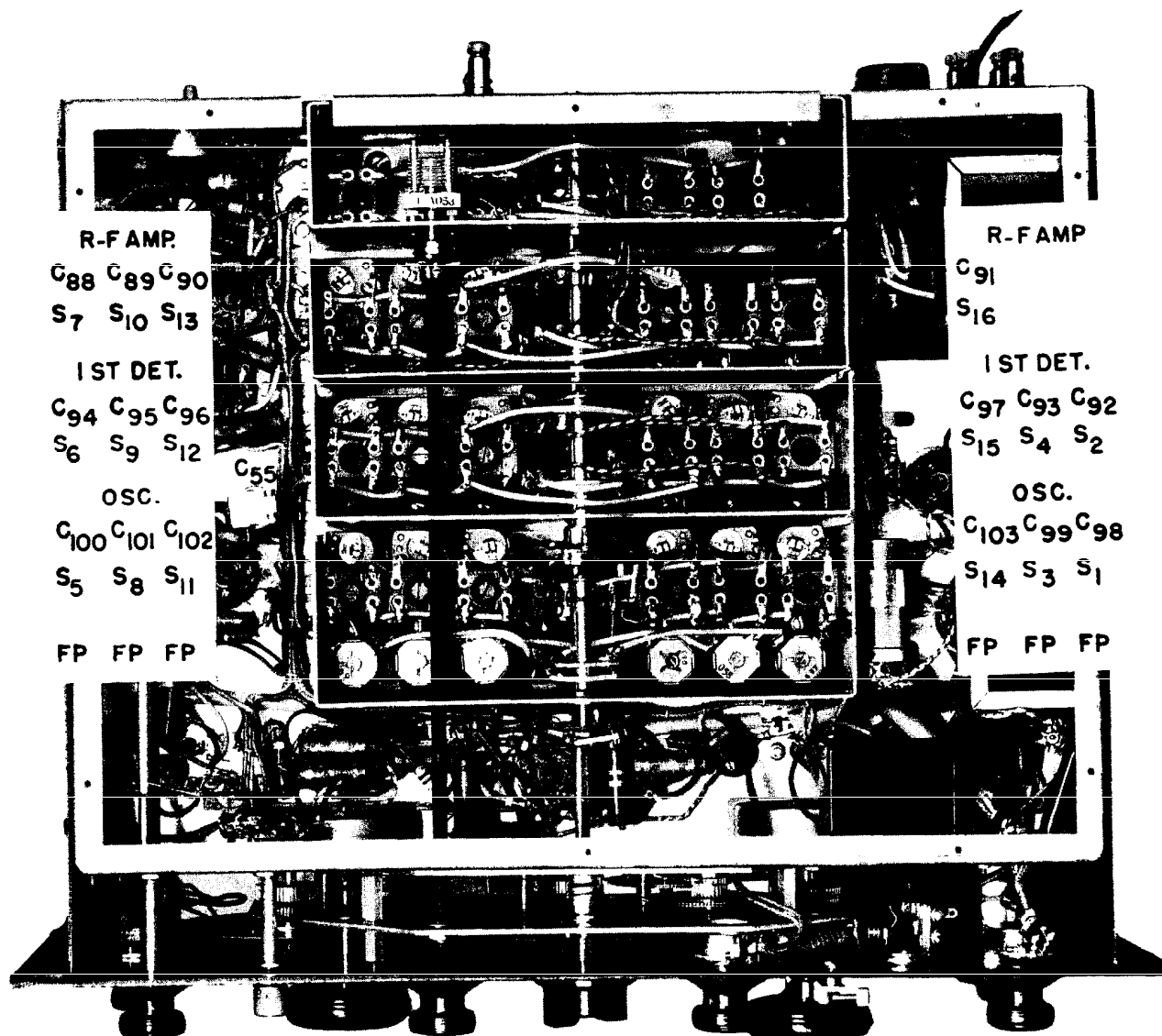
FIG. 12—RF AND OSC ADJUSTMENT LOCATION AND ALIGNMENT PROCEDURE
