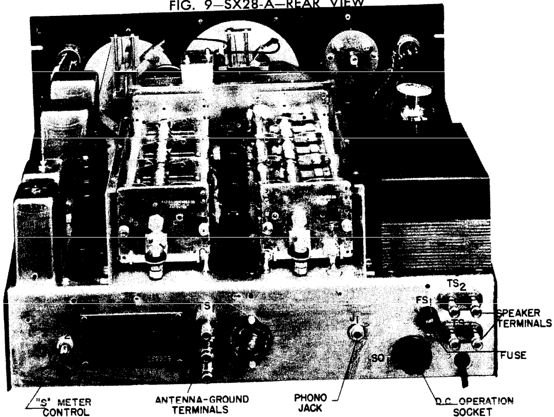
FIG. 9—SX28-A—REAR VIEW
