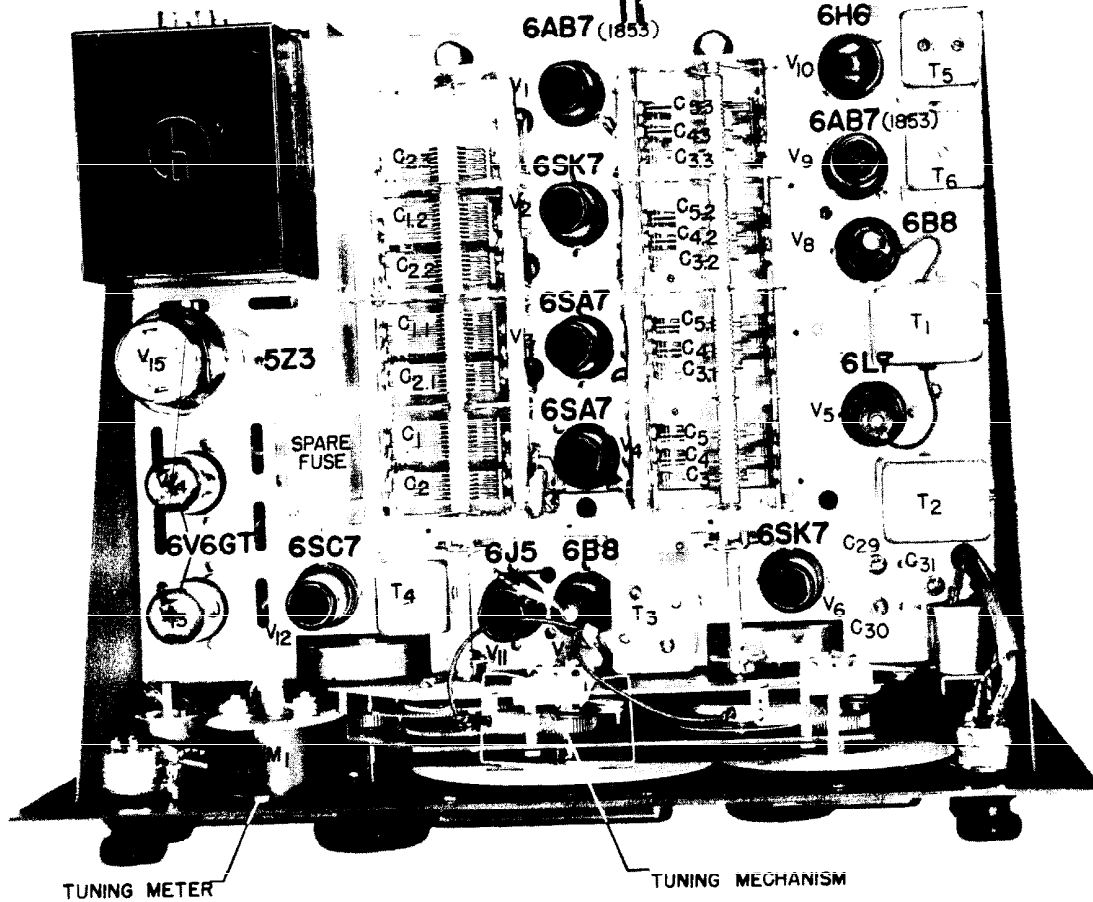
FIG. 9—SX28-A—REAR VIEW
