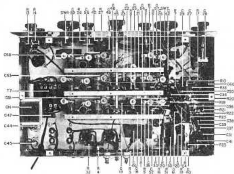
Bottom View
