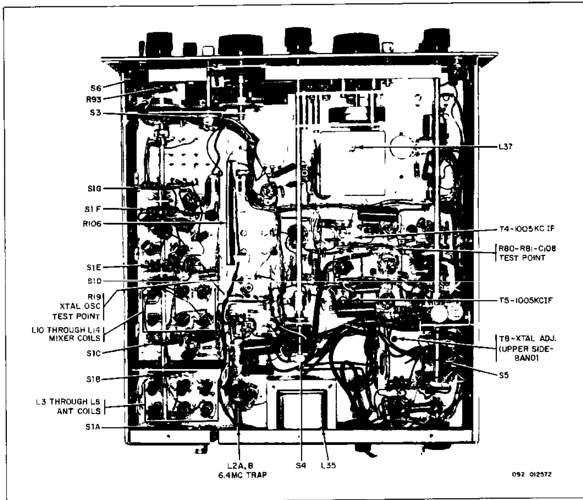
Figure 10. Bottom Chassis View of Receiver.
