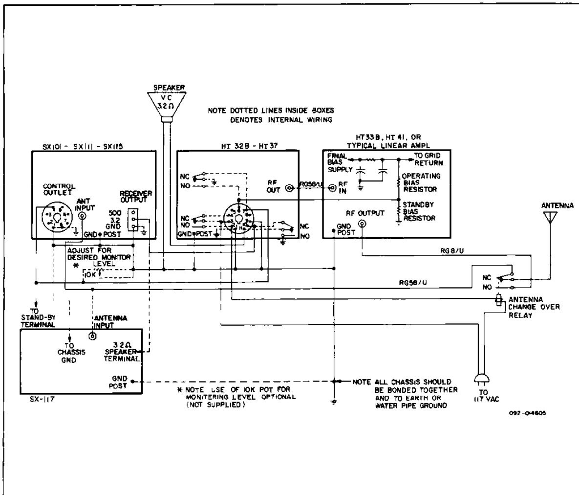
Figure 16. Typical Station Setup.
