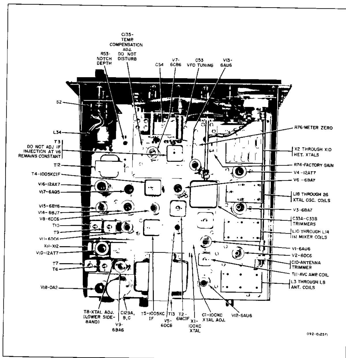
Figure 9. Top Chassis View of Receiver.
