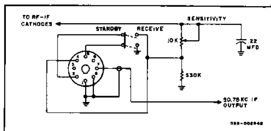
Figure 4. Sensitivity and Receive-Standby Circuit.
