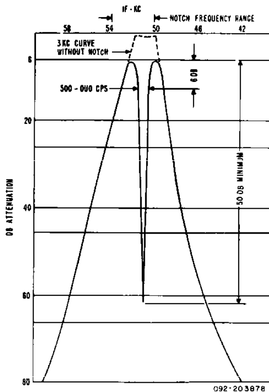
Figure 7. IF Selectivity with Notch.
