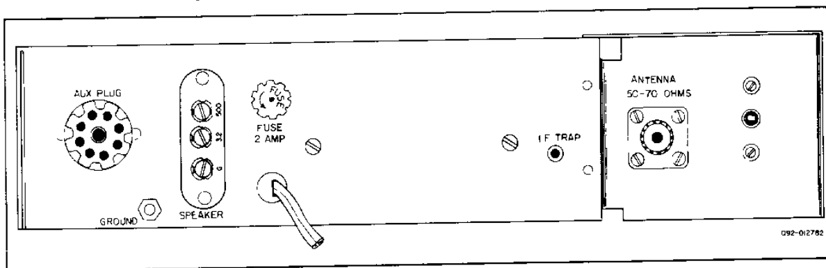
Figure 3. Rear View of Receiver.
