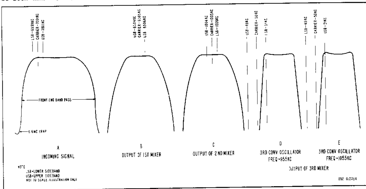
Figure 8. Selectable Sideband Response Curves.
