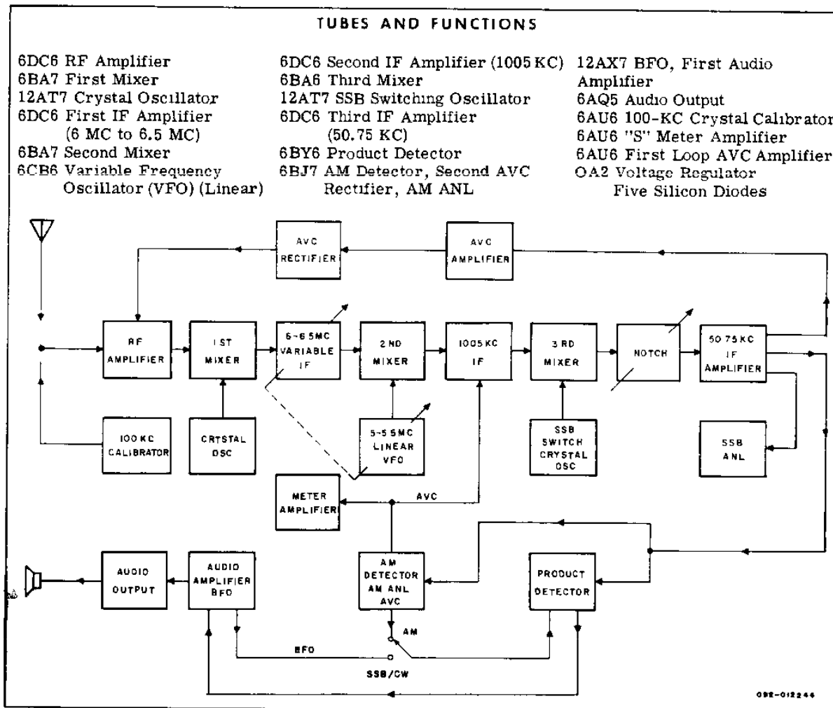
Figure 1. Block Diagram of Receiver.
