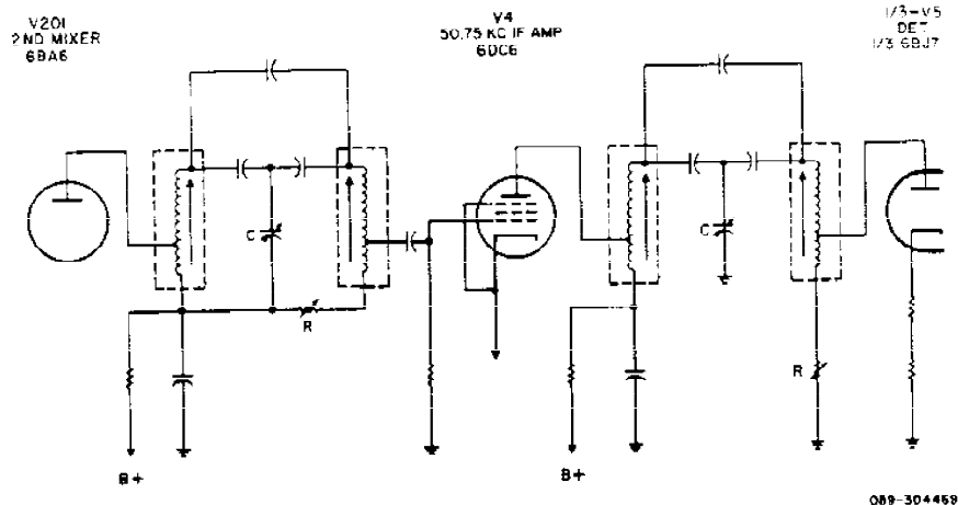
Figure 12. Equivalent Schematic Diagram of 50.75KC IF System
