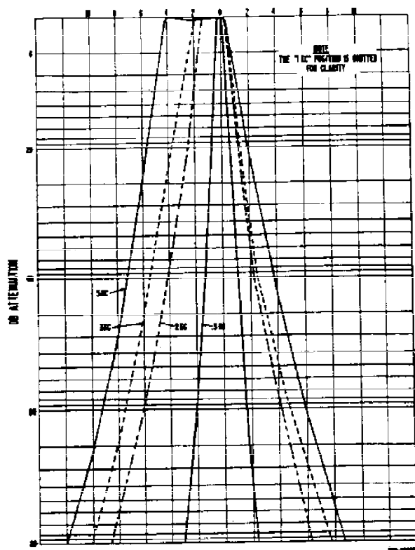
Figure 7. IF Selectivity Curves
