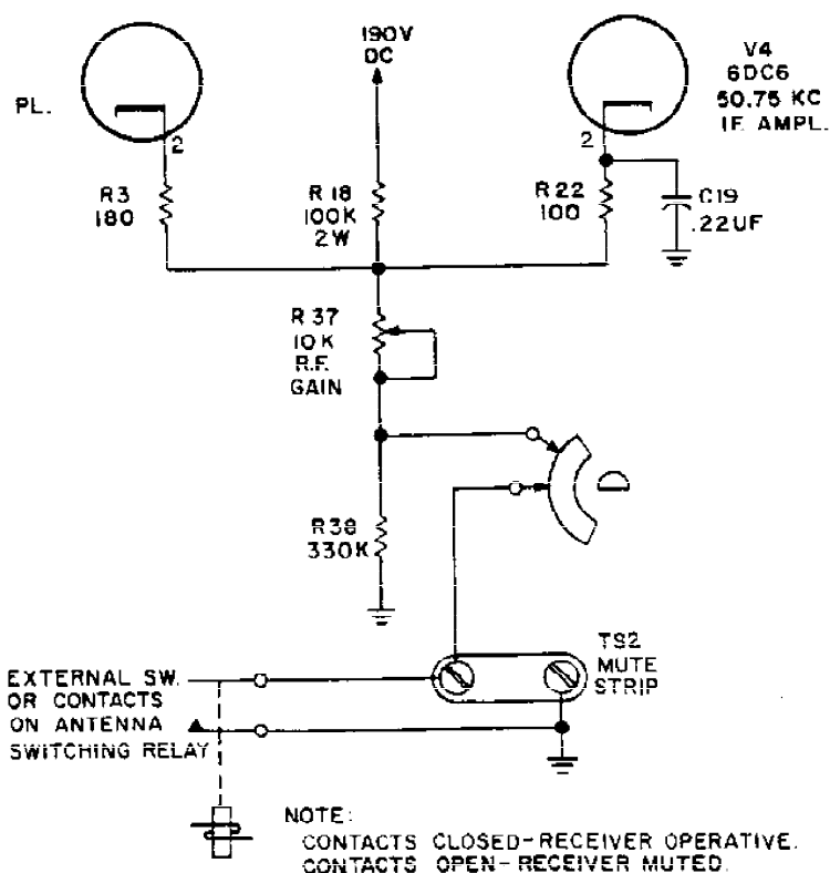
Figure 5. Schematic Diagram of Remote Receive-Standby Circuitry
