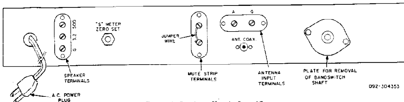
Figure 4. Receiver Chassis Rear View
