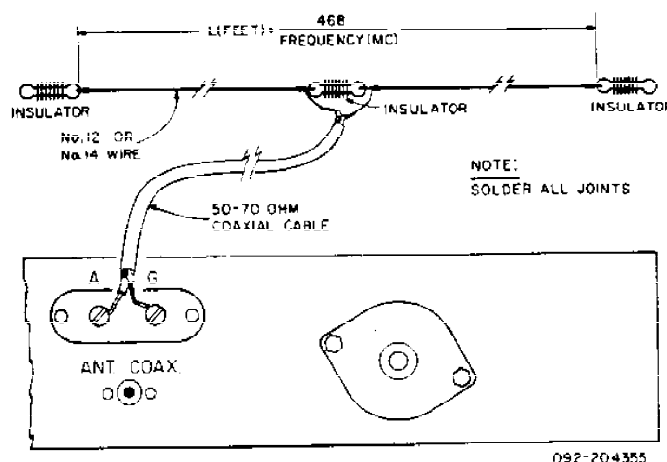
Figure 3. Doublet Antenna Using Twin-Lead Transmission Line
