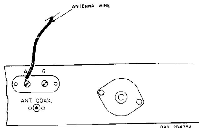
Figure 2. Single Wire Antenna
