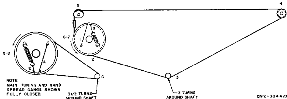
Figure 6. Dial Cord Stringing Diagram
