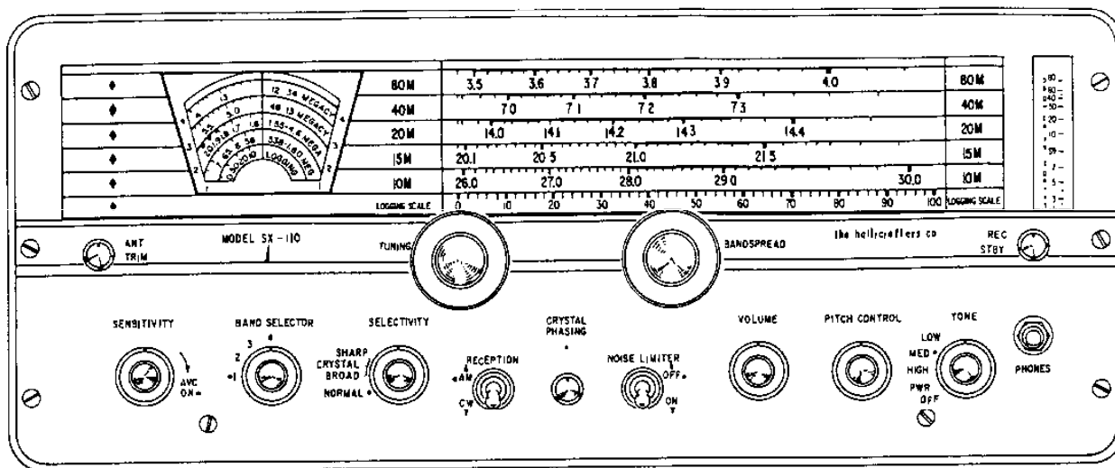
Figure 4. Operating Controls
