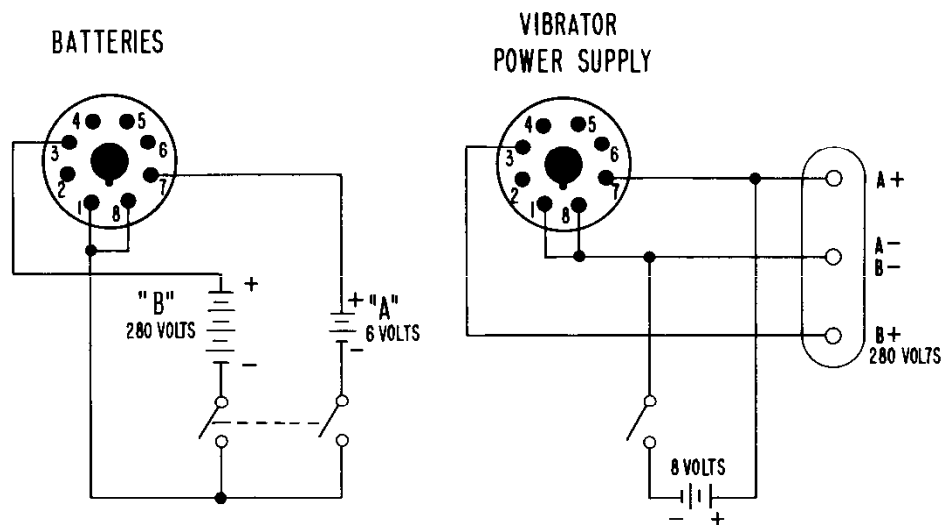
Fig. 5. Wiring Diagram for DC Operation
