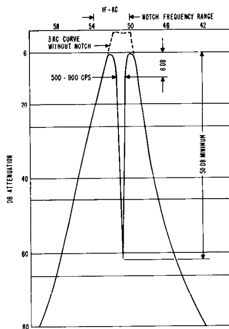
Fig. 9. IF Selectivity Curve with Notch
