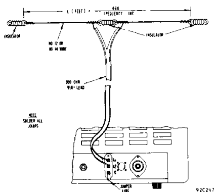
Fig.-3. Doublet Antenna Using Twin-Lead Transmission Line
