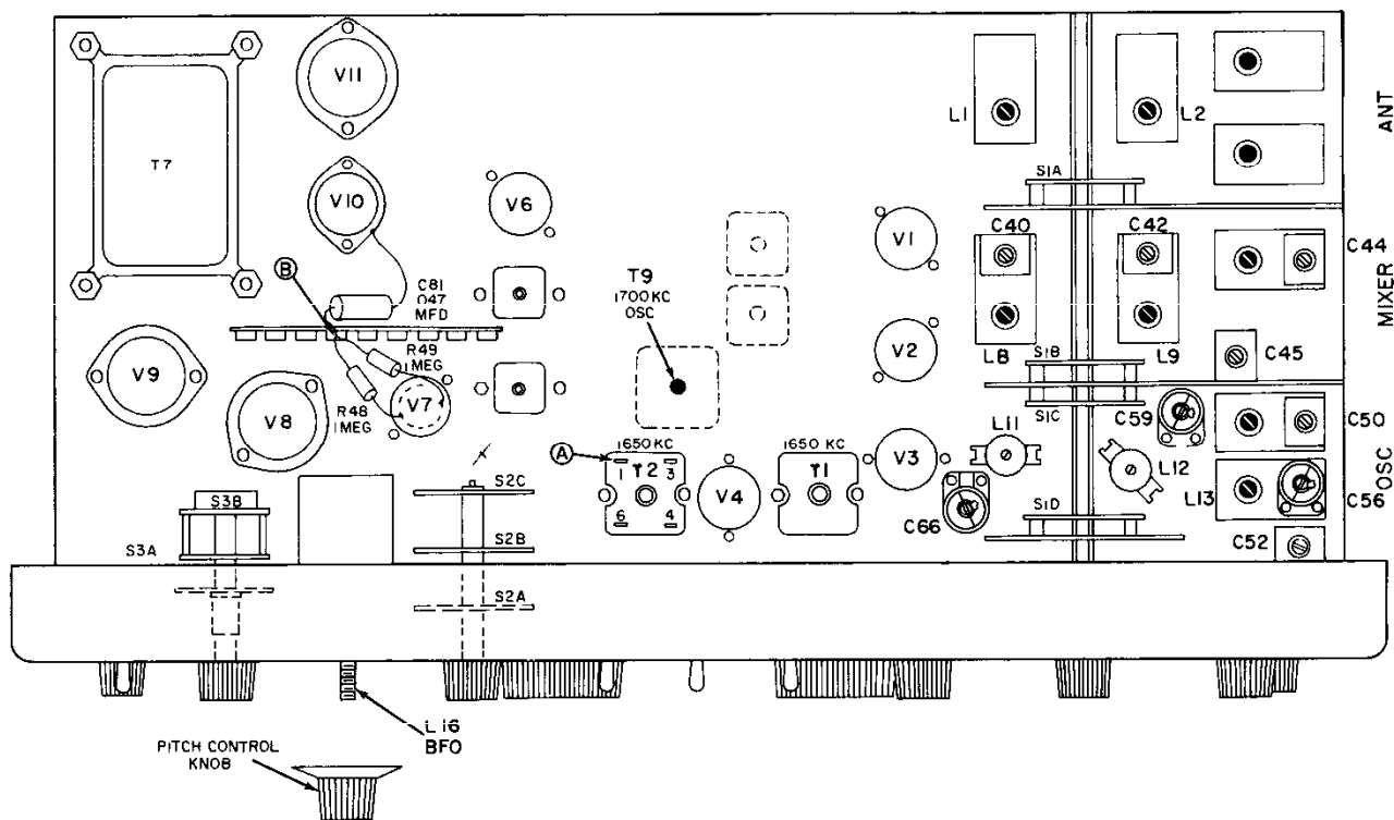
Figure 12. Bottom View of Chassis Showing Location of Alignment Adjustments and Tubes
