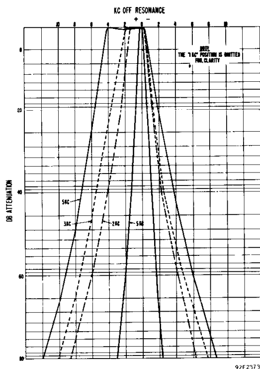
Fig. 8. IF Selectivity Curves
