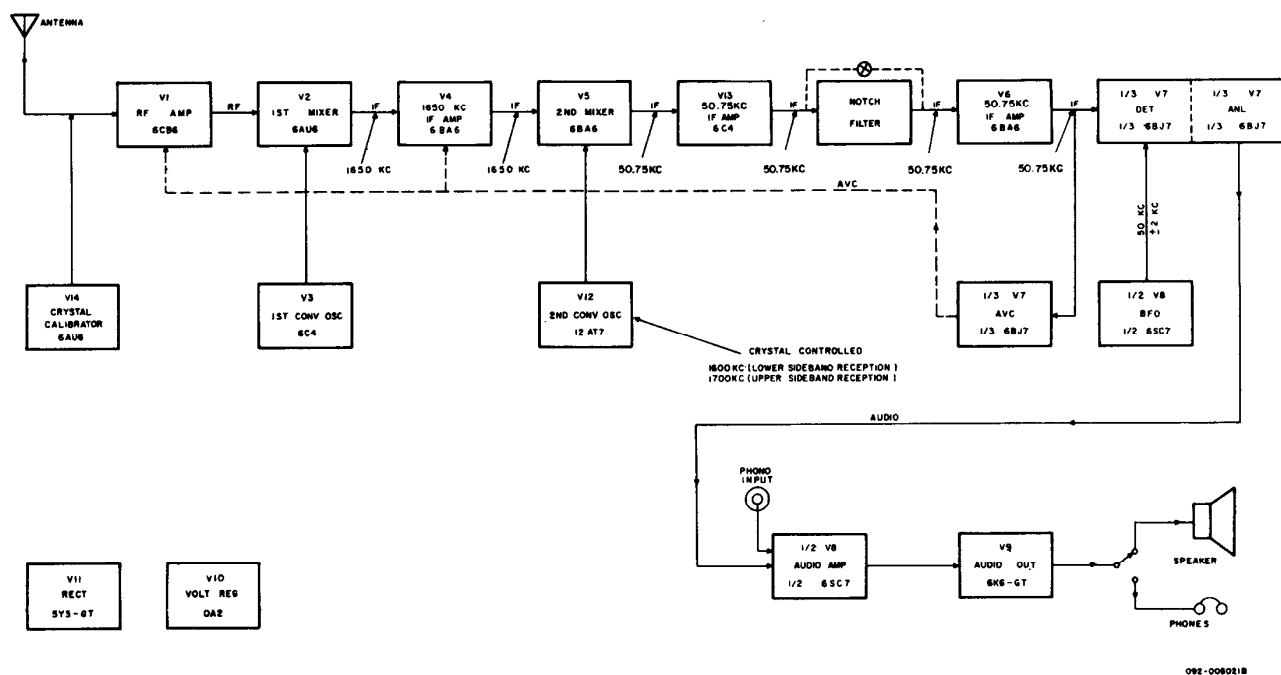
Figure 16. Block Diagram of Receiver
