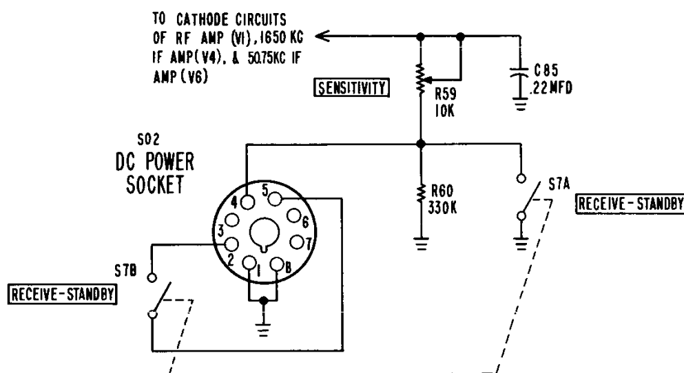
Figure 6. Schematic Diagram of Sensitivity and Receive-Standby Circuits.
