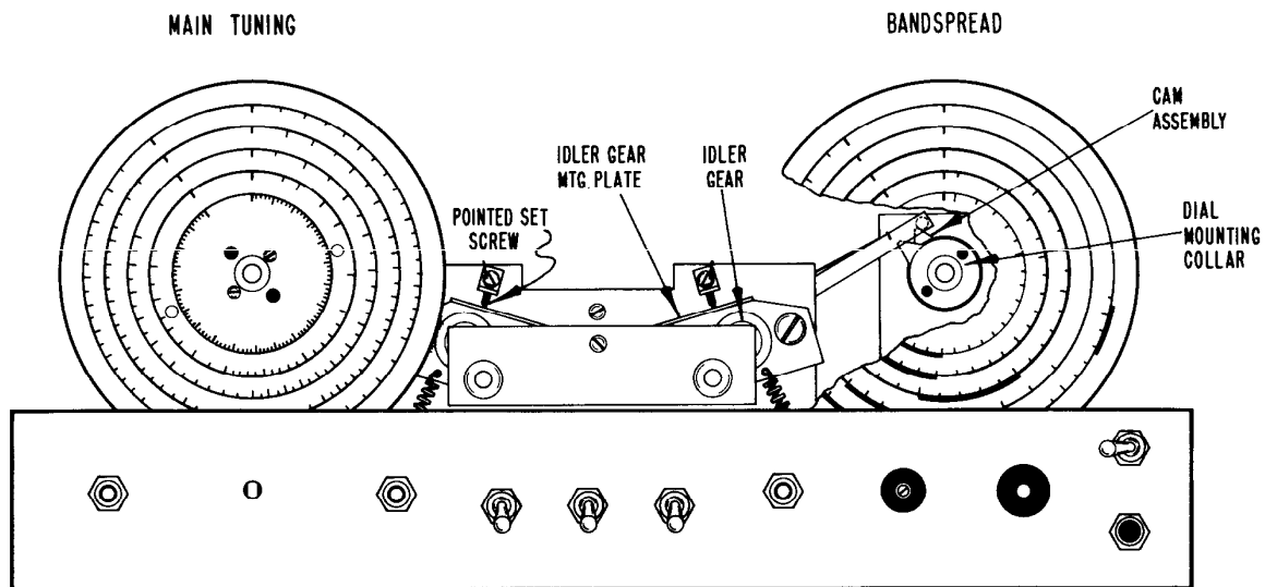
Fig. 15. Front View of Gear Drive Tuning Mechanism
