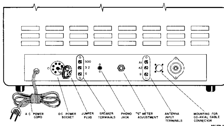
Fig. 4. Rear View of Receiver
