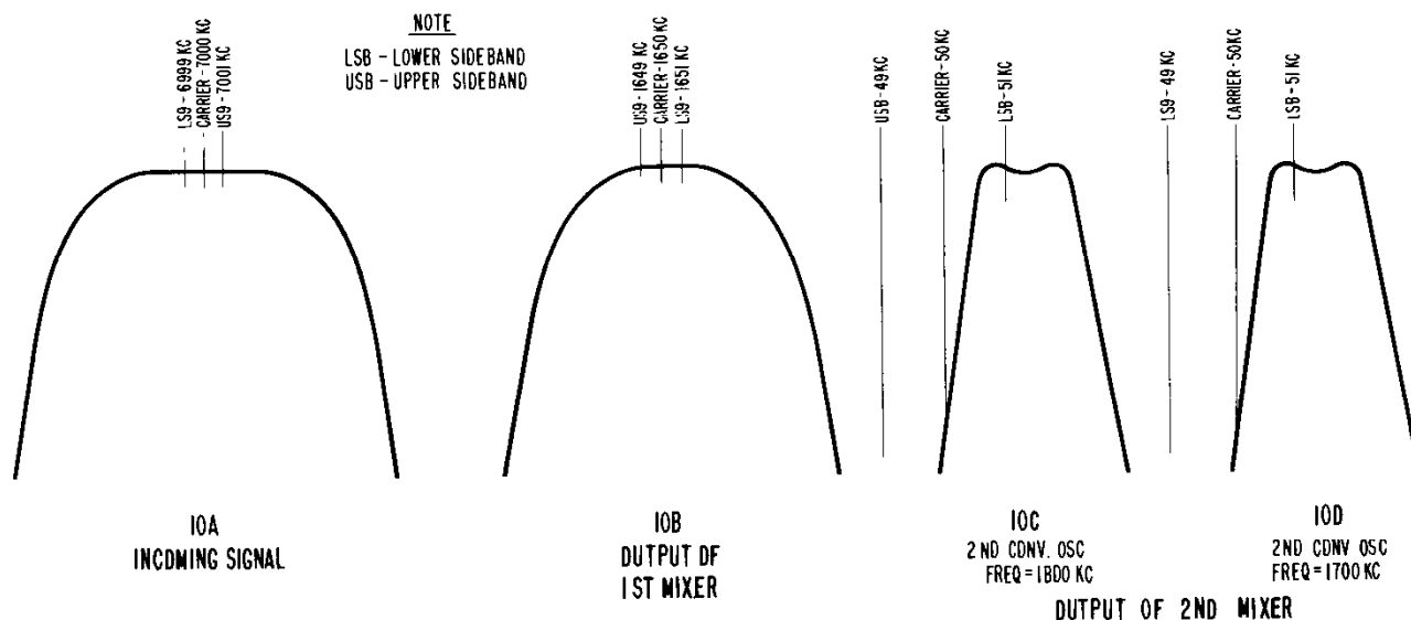
Figure 10. IF Selectable-Sideband Response Curves
