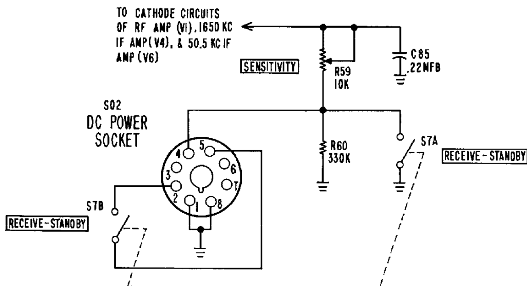
Fig. 6. Schematic Diagram of Sensitivity and Receive-Standby Circuits
