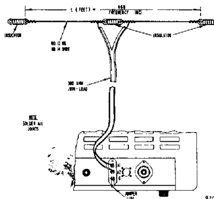
Fig. 3. Doublet Antenna Using Twin-Lead Transmission Line
