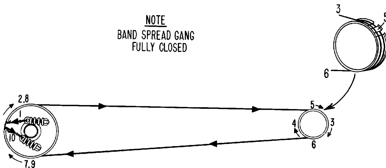
Fig. 14. Dial Cord Stringing Diagram
