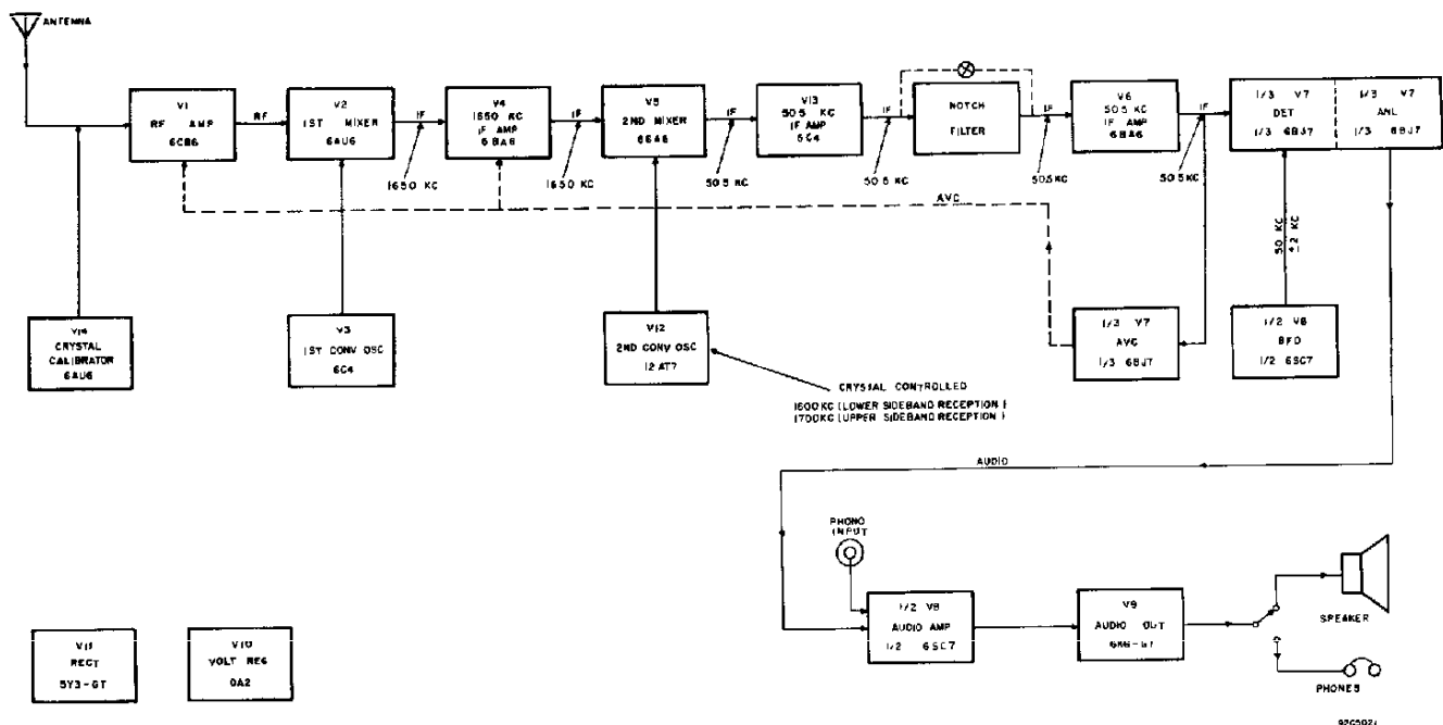
Fig. 16. Block Diagram of Receiver
