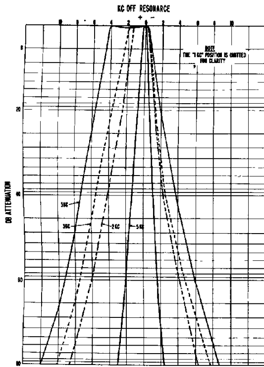
Fig. 8. IF Selectivity Curves
