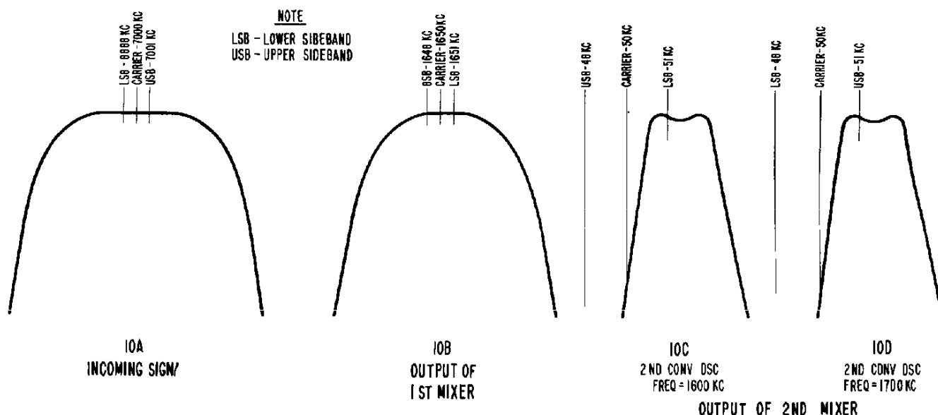
Fig. 10. Selectable-Sideband Response Curves
