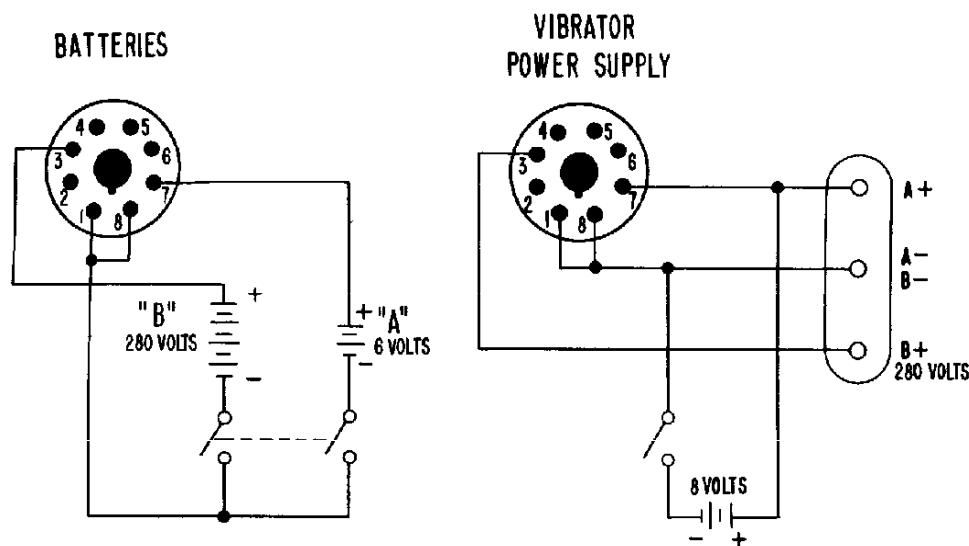
Fig. 5. Wiring Diagram for DC Operation
