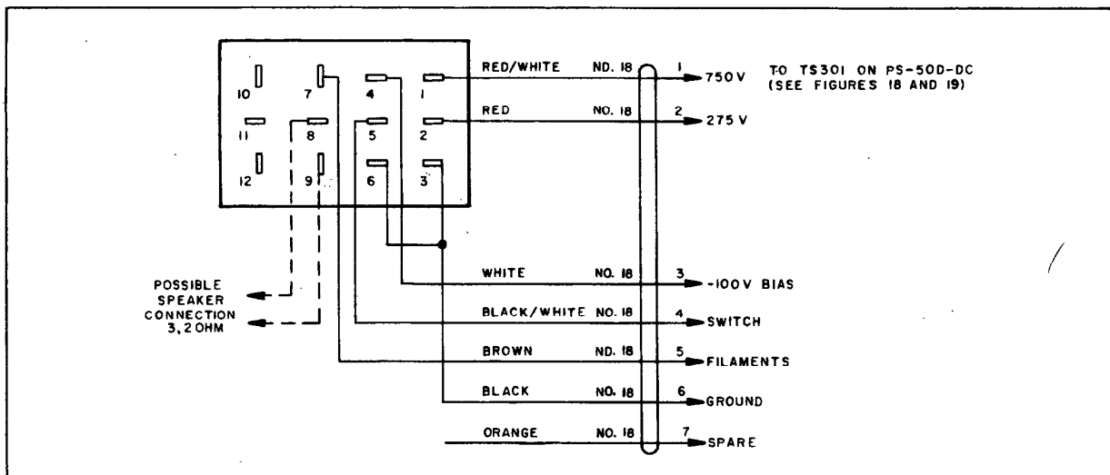
Figure 7. Schematic Diagram of Model MR-160 Interconnecting Cable.
