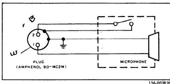
Figure 8. Required Microphone Wiring.
