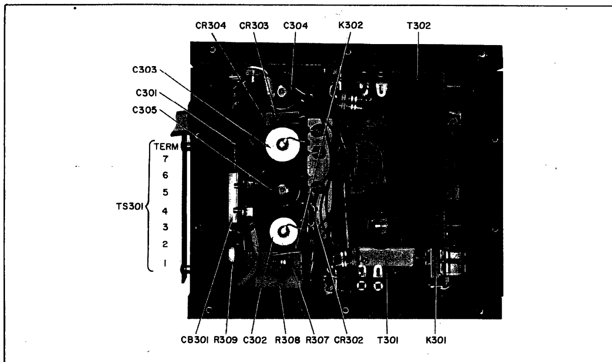
Figure 18. Internal View of Model PS-500-DC Power Supply.
