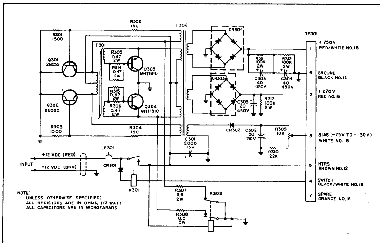
Figure 19. Schematic Diagram of Model PS-500-DC Power Supply.
