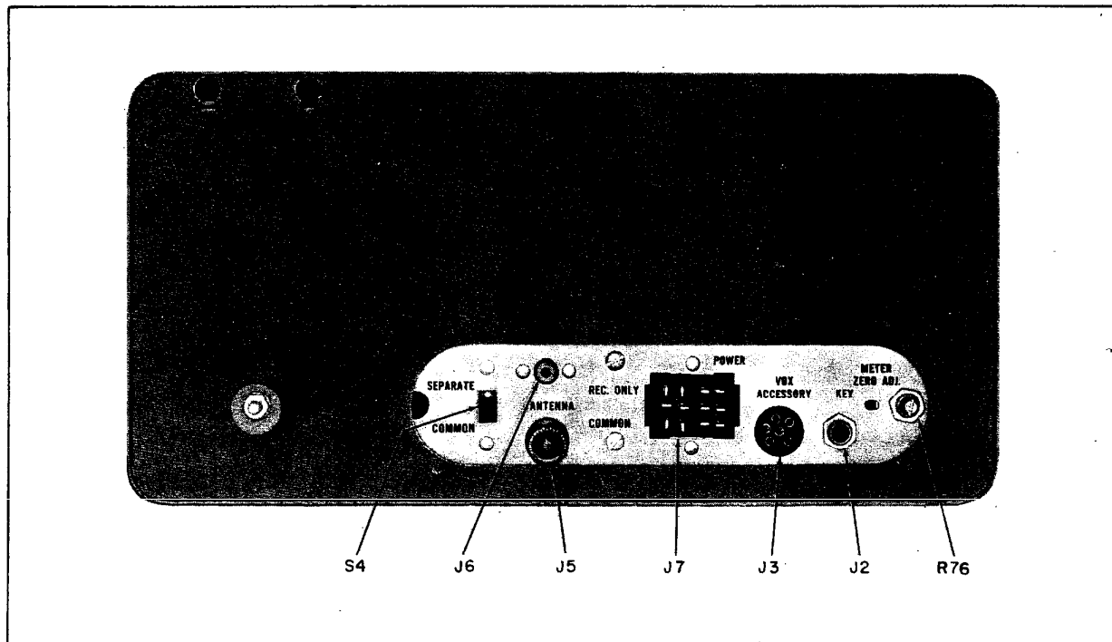
Figure 2. Rear Panel View of Transceiver.
