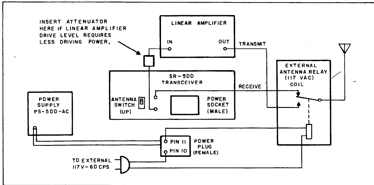
Figure 3. Base Installation, Using a Linear Amplifier.
