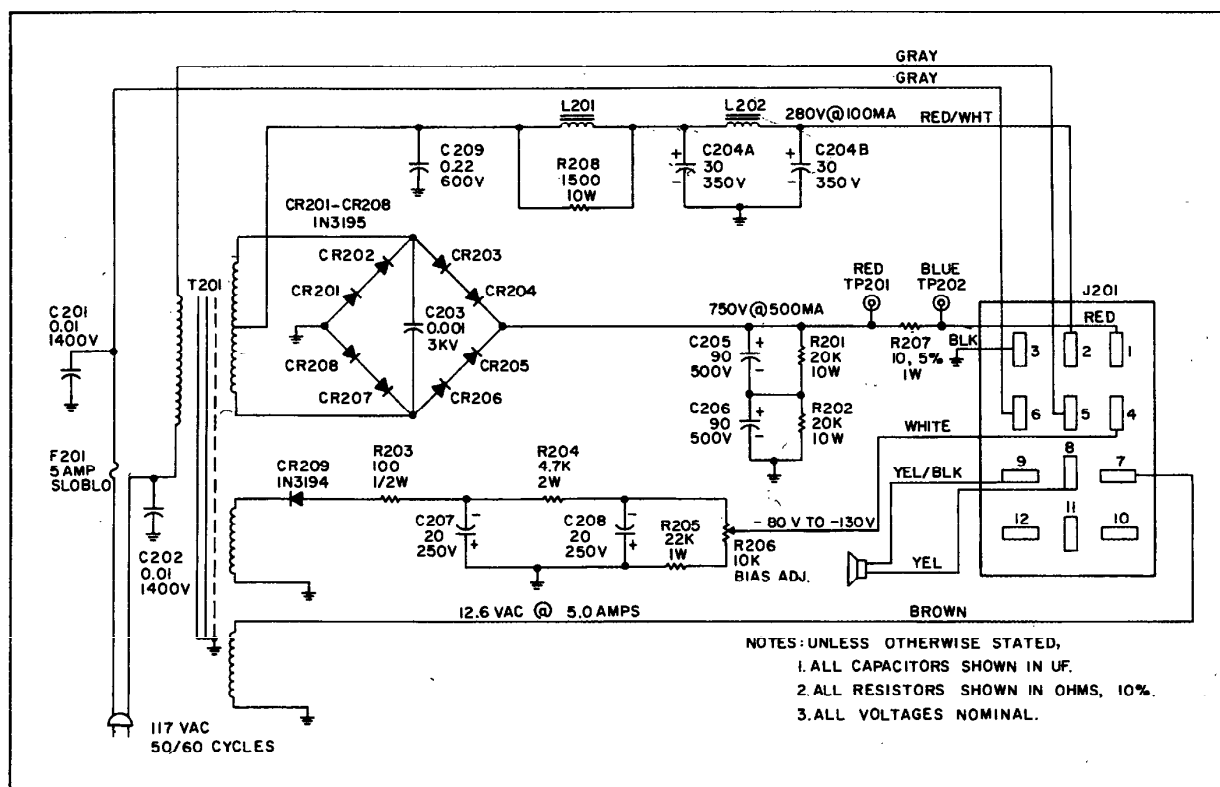
Figure 16. Schematic Diagram of Model PS-500-AC Power Supply.
