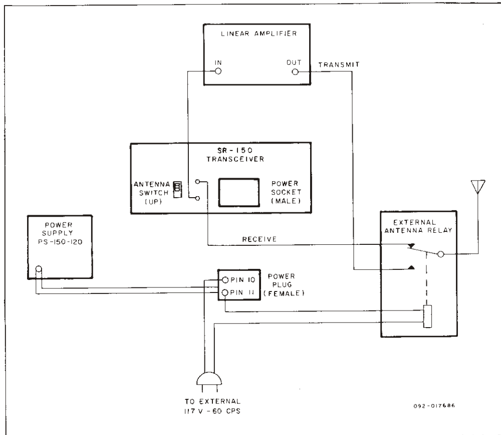
Figure 3. Base Installation Using a Linear Amplifier.
