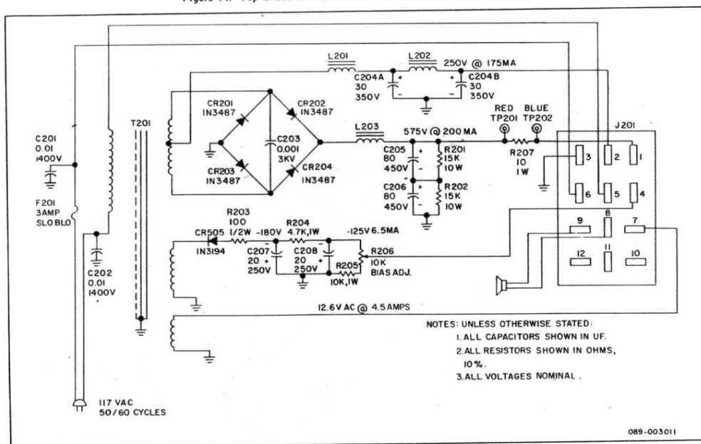
Figure 15. Schematic Diagram of Model PS-150-120 AC Power Supply.
