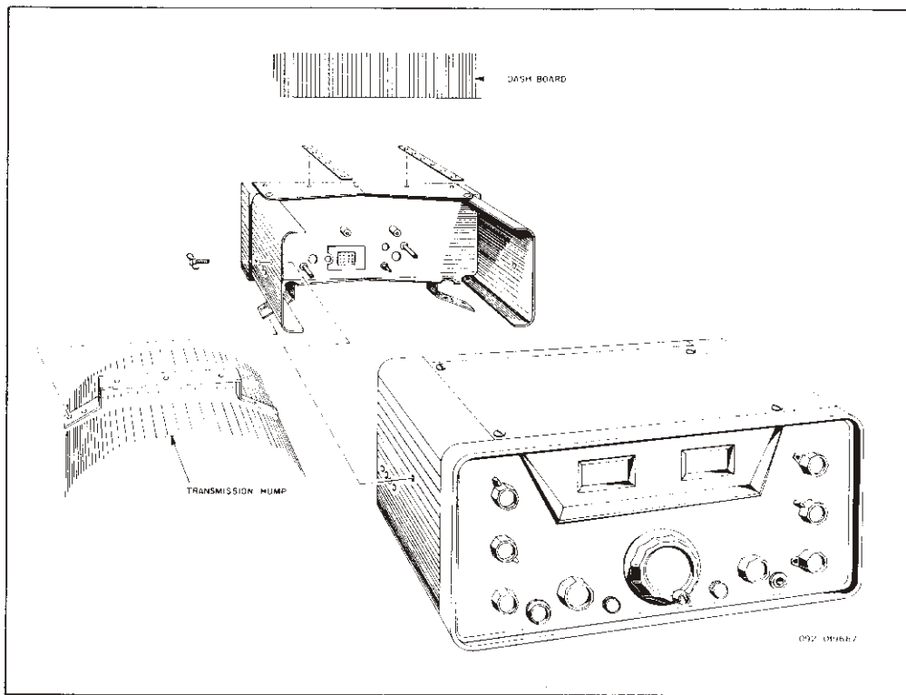
Figure 4. Installing the Model MR-150 Mounting Rack.
