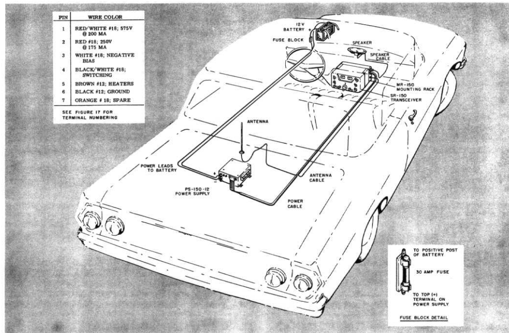
Figure 5. Wiring Diagram of Mobile Installation.
