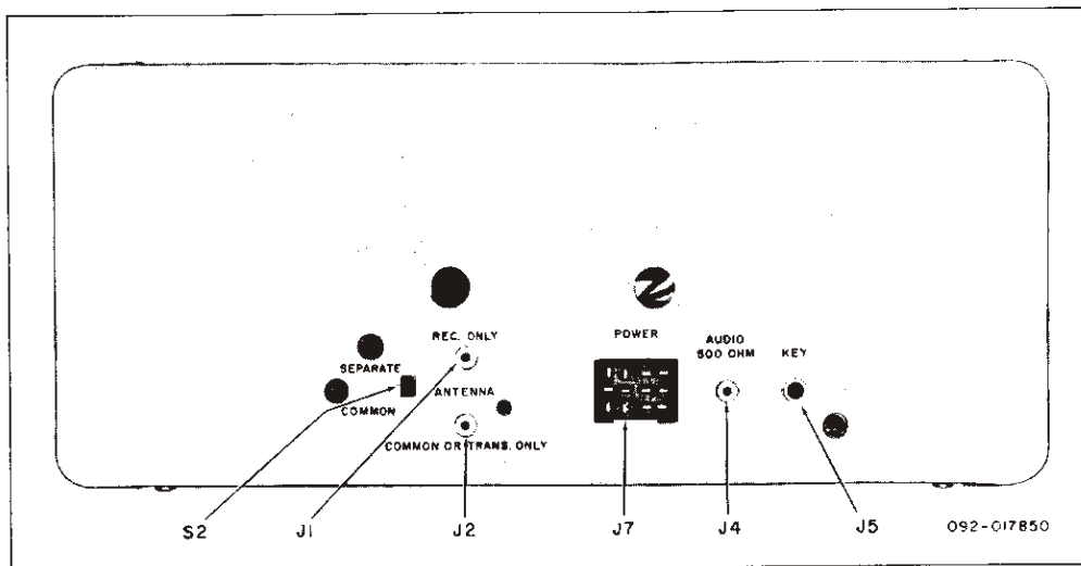
Figure 2. Rear View of Transceiver.
