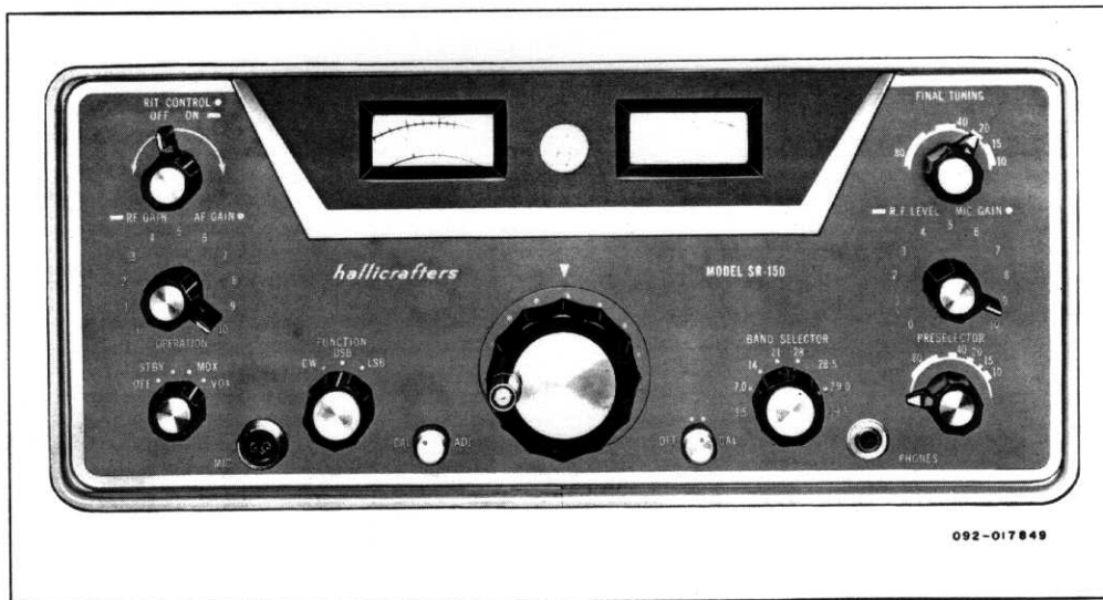
Figure 7. Front Panel View of Transceiver.
