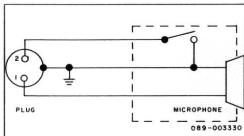
Figure 6. Required Microphone Wiring.
