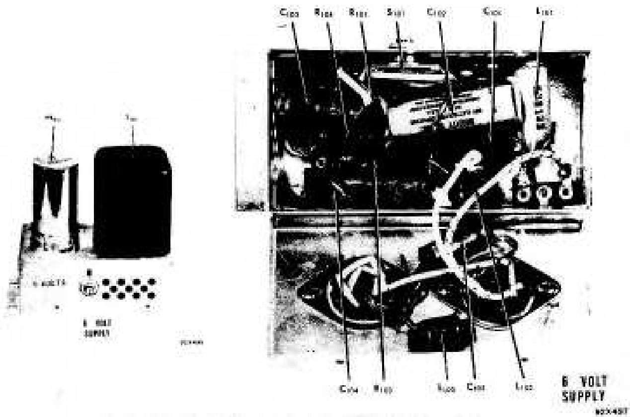
FIG. 6. Component location, 6-volt adapter unit. (927450 & 927497)
