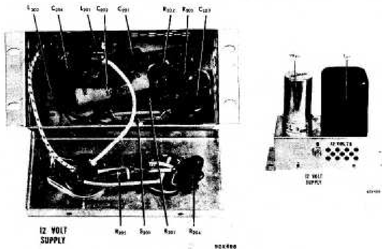
Fig. 7. Component location, 12-volt adapter unit.
