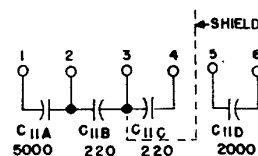
Fig. 9. Schematic Diagram
