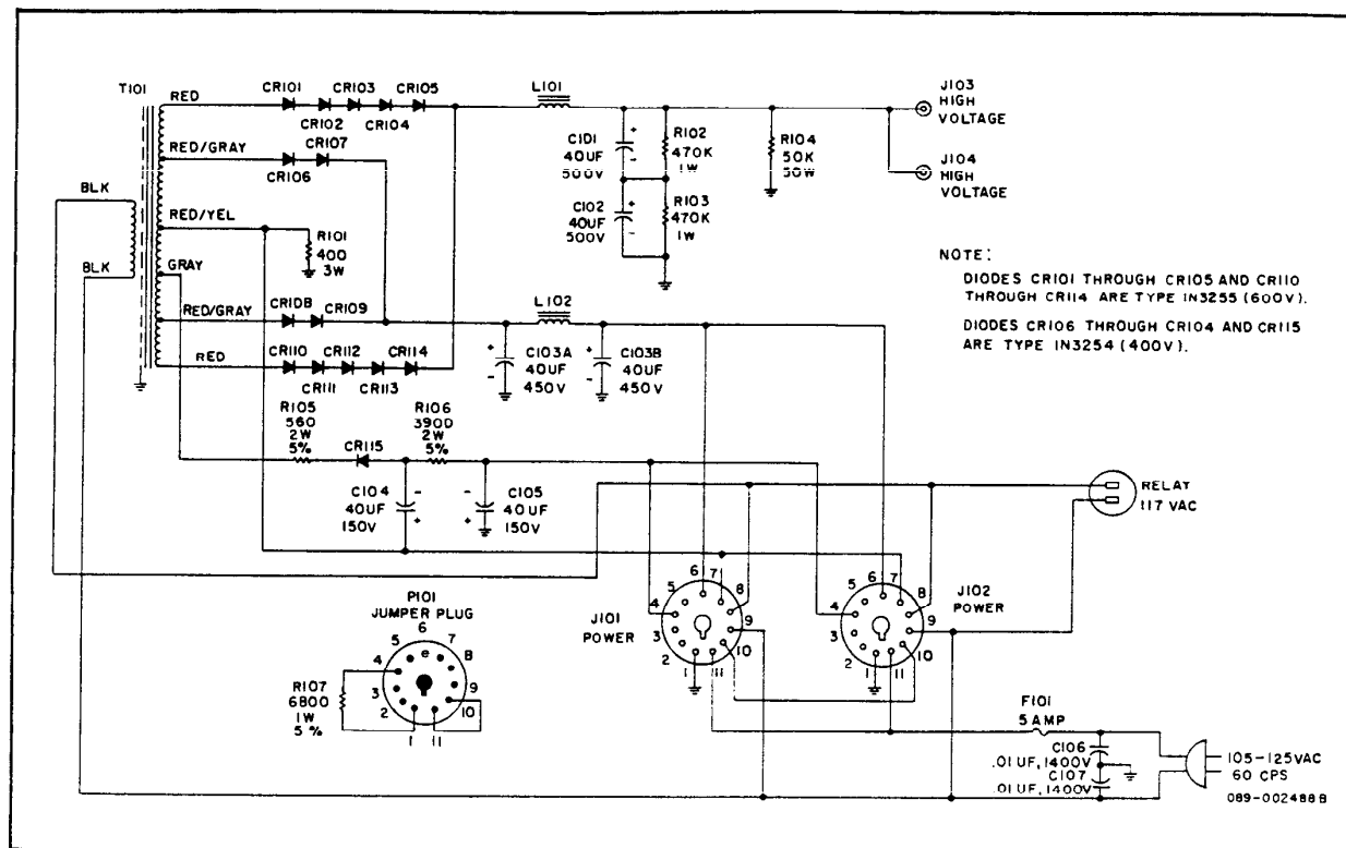
Figure 15. Schematic Diagram of Model P-26 Power Supply.
