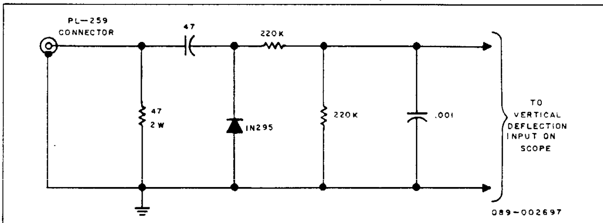
Figure 11. Diode Detector.
