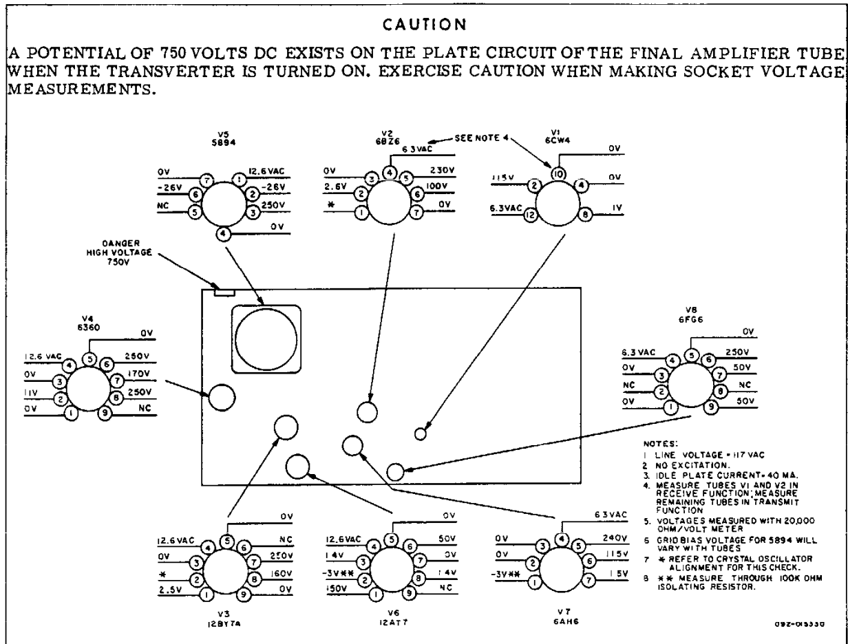
Figure 7. Voltage Chart.
