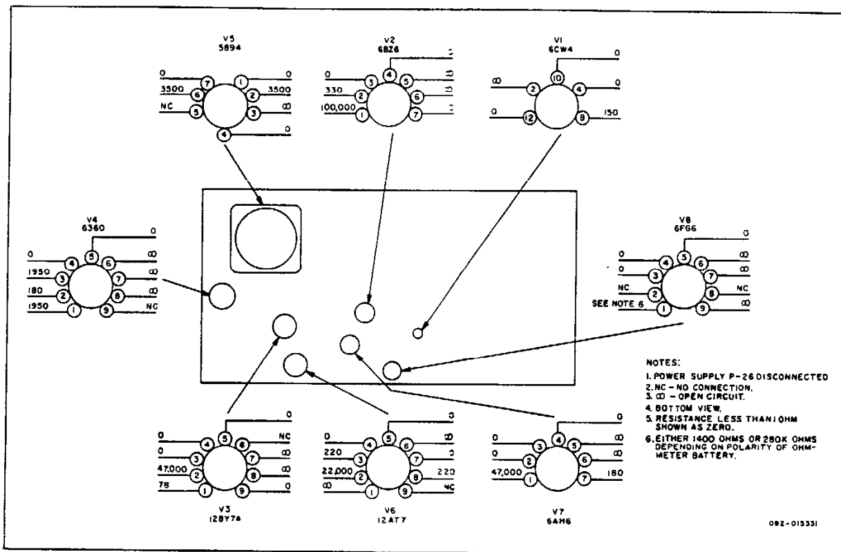
Figure 8. Resistance Chart.
