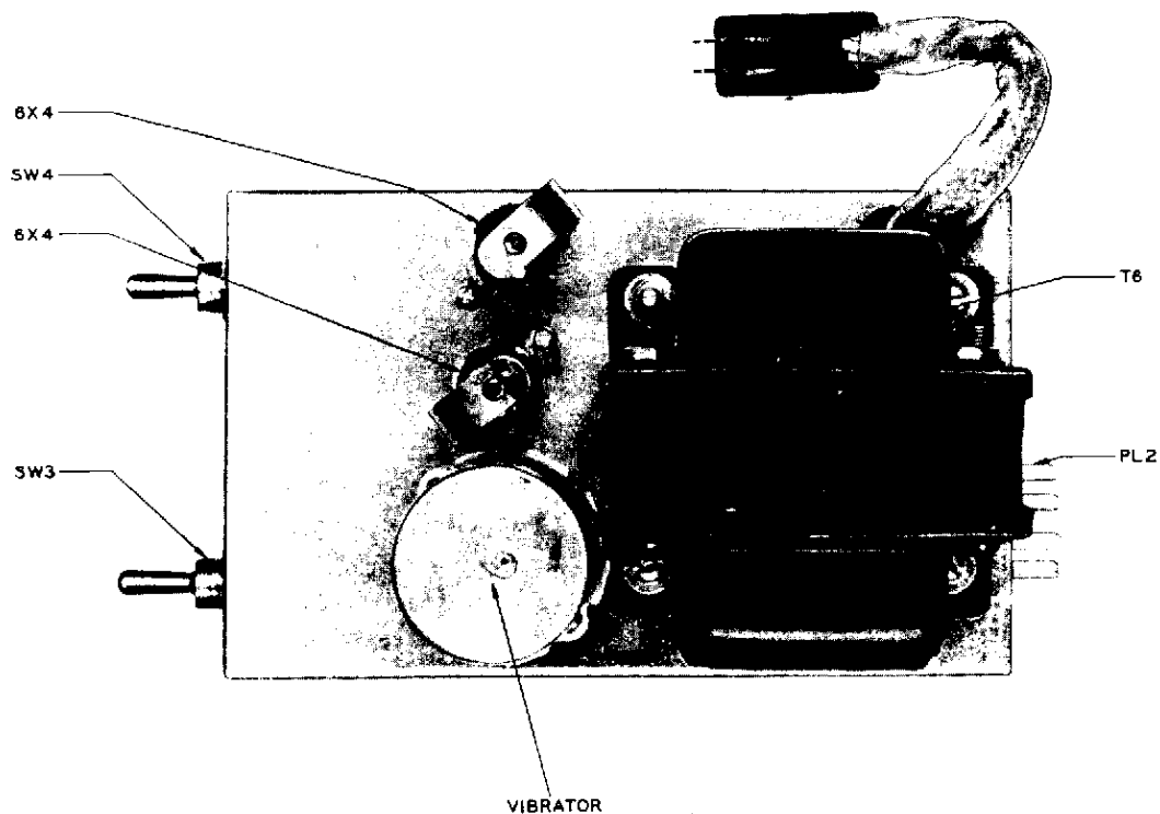
TOP VIEW - POWER SUPPLY
