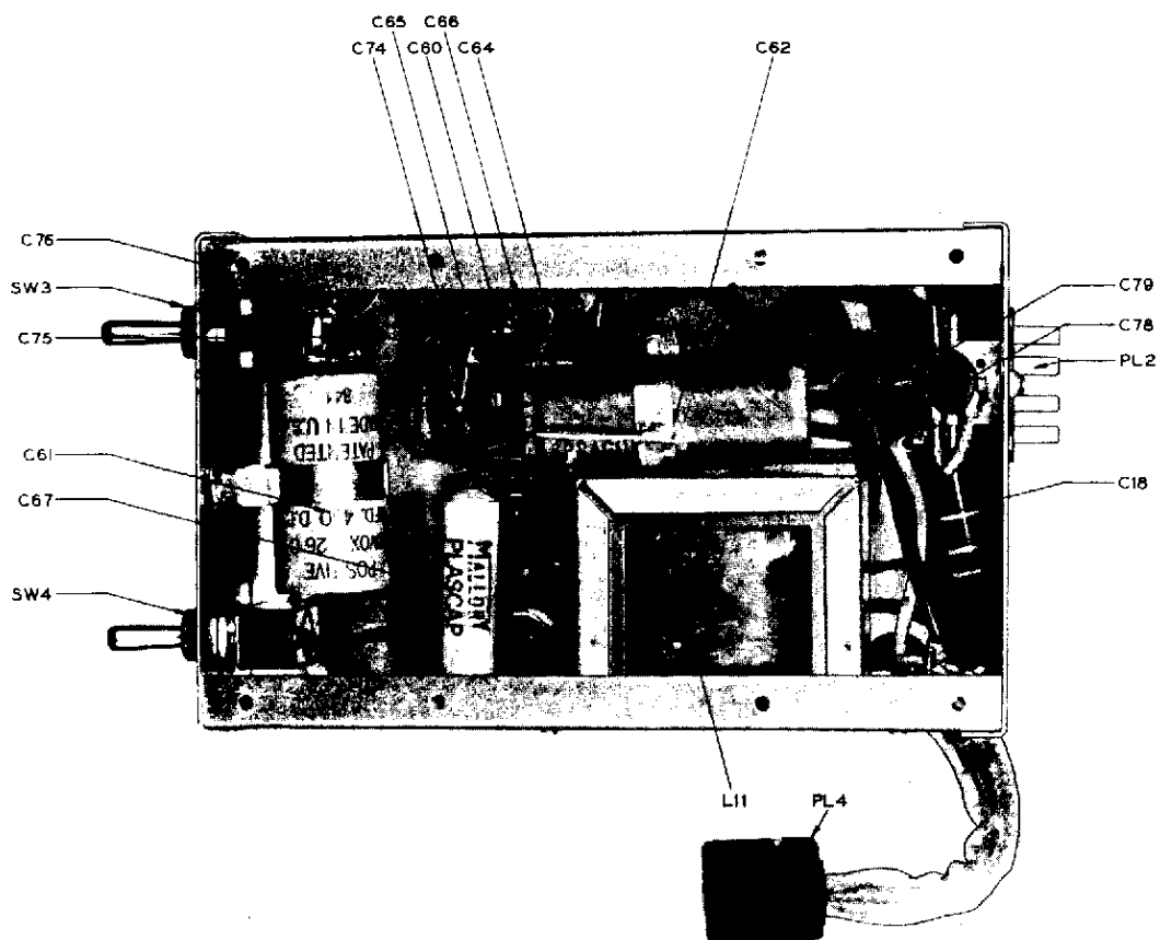
BOTTOM VIEW - POWER SUPPLY
