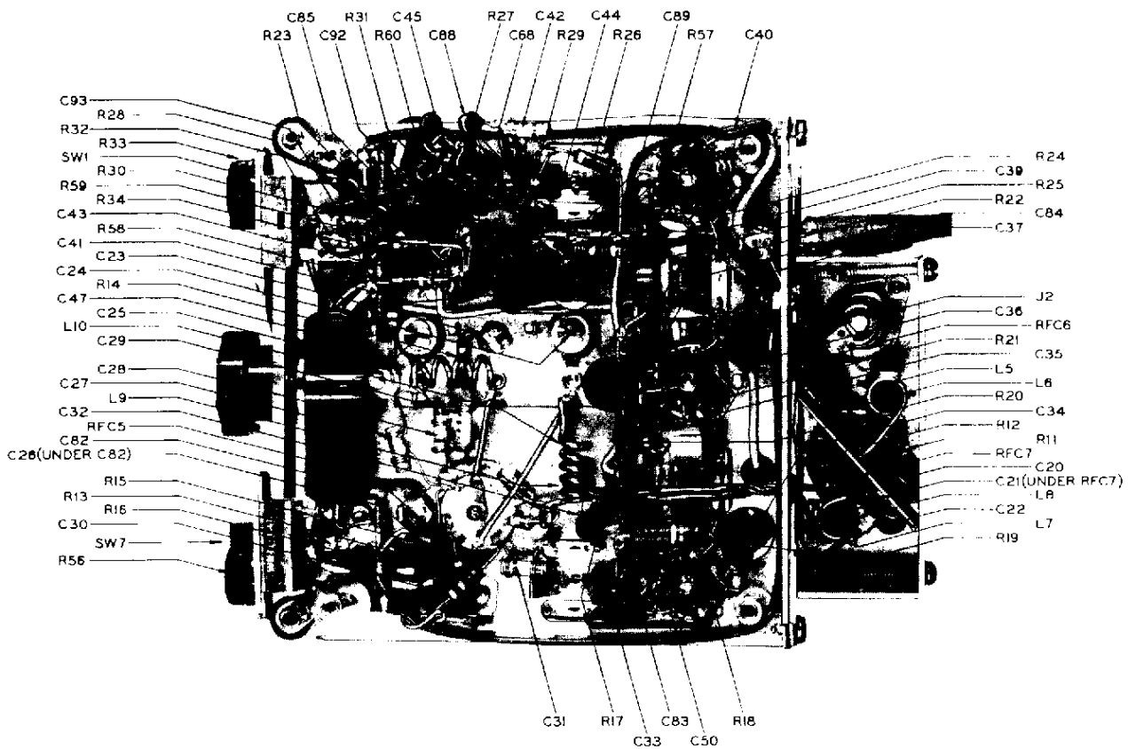
BOTTOM VIEW - RECEIVER
