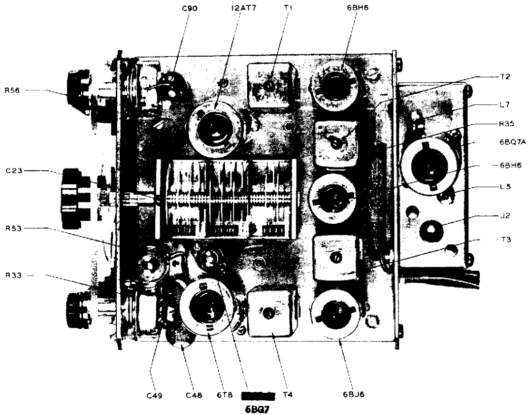
TOP VIEW - RECEIVER
