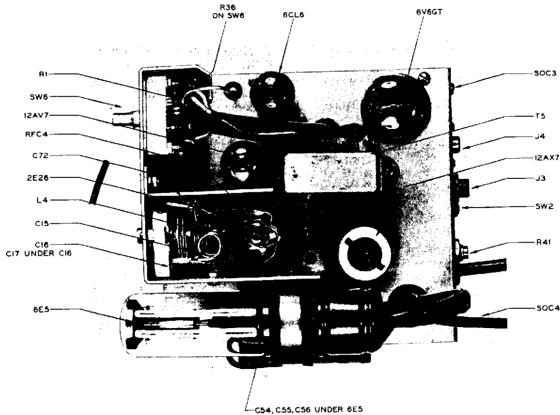
TOP VIEW - TRANSMITTER
