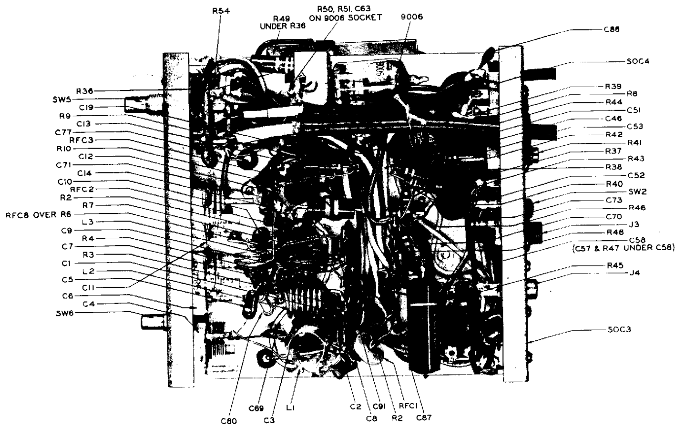
BOTTOM VIEW - TRANSMITTER
