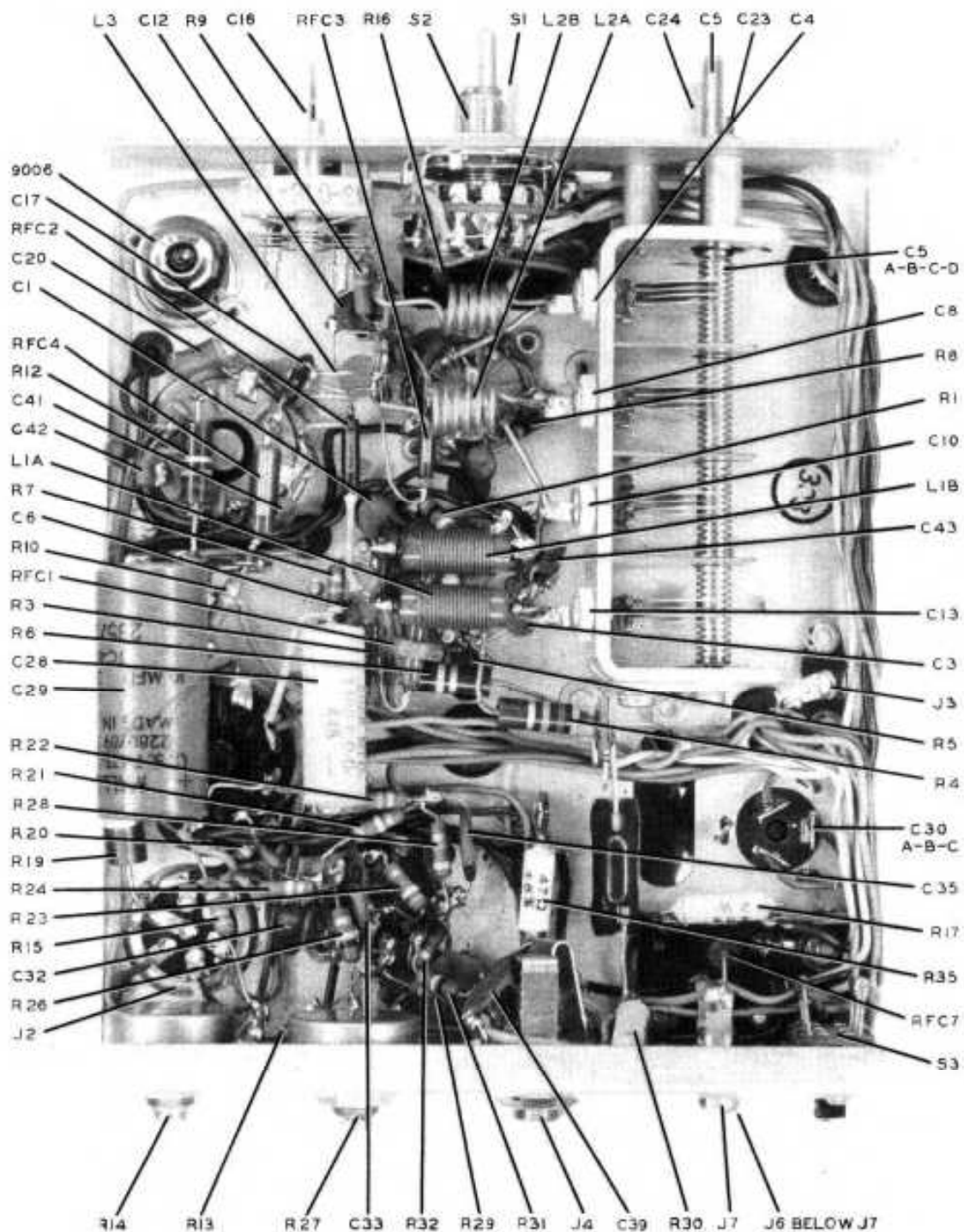
2 METER TRANSMITTER — BOTTOM VIEW
