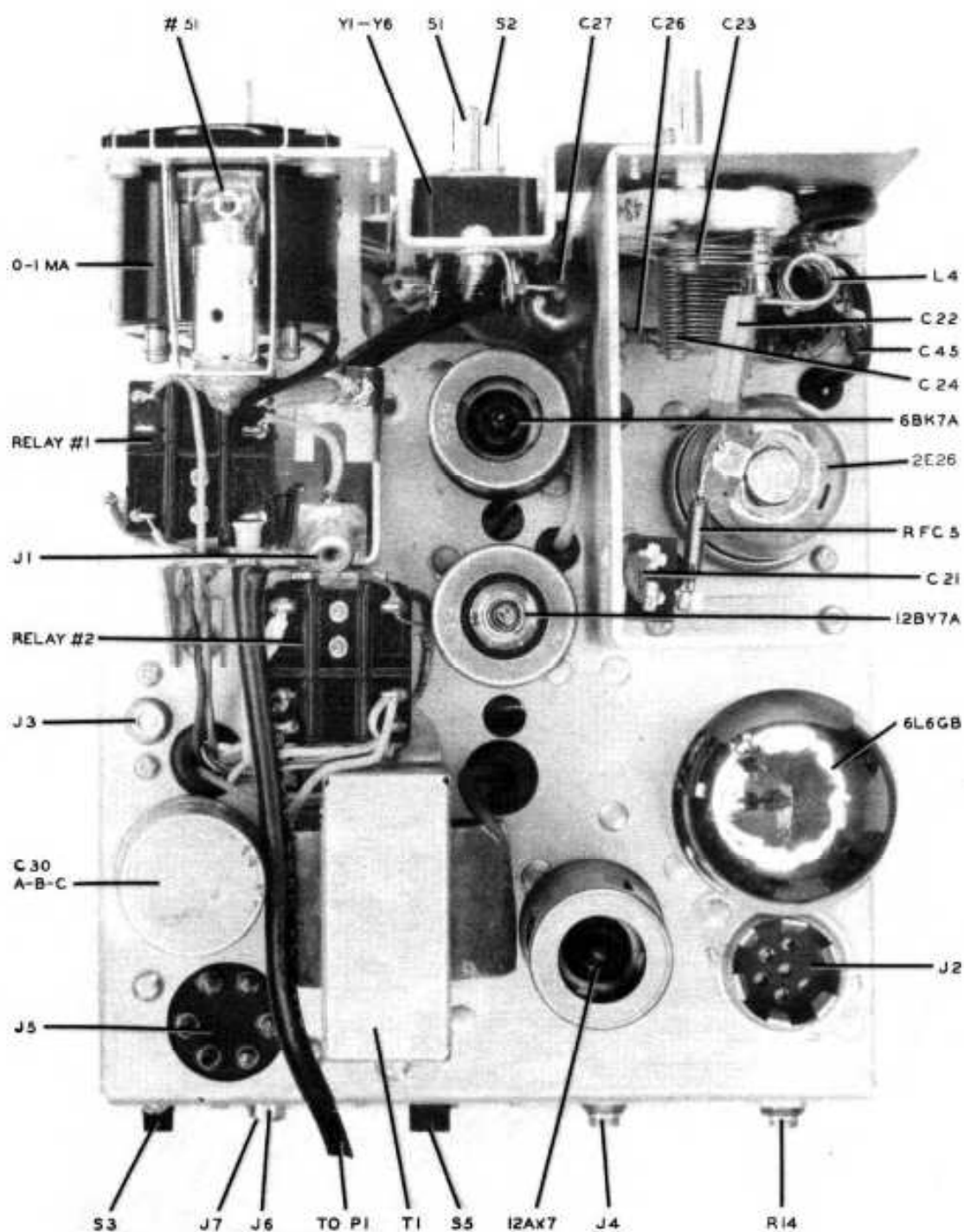
TRANSMITTER — TOP VIEW
