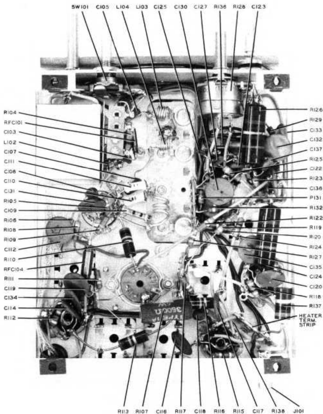
2 METER RECEIVER — BOTTOM VIEW
