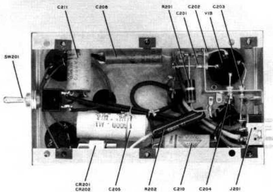
POWER SUPPLY — BOTTOM VIEW
