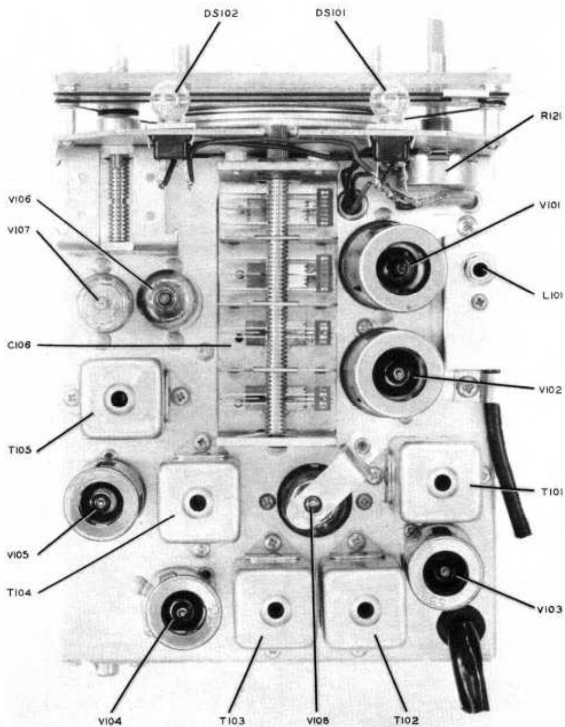
RECEIVER — TOP VIEW
