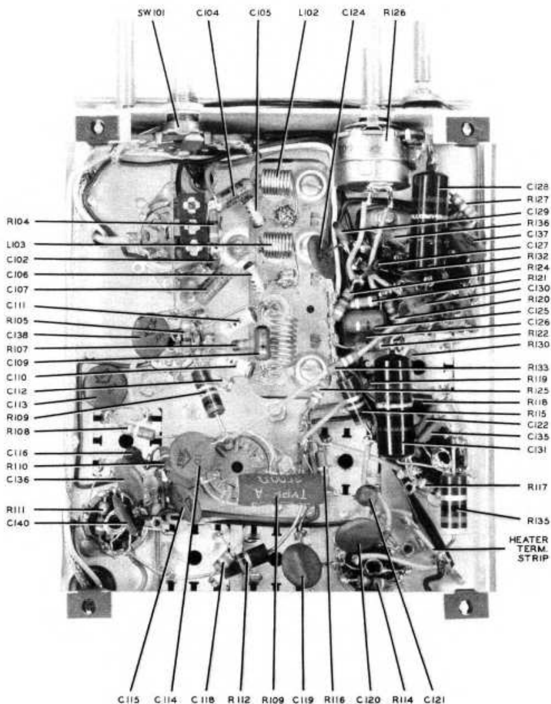
6 METER RECEIVER — BOTTOM VIEW
