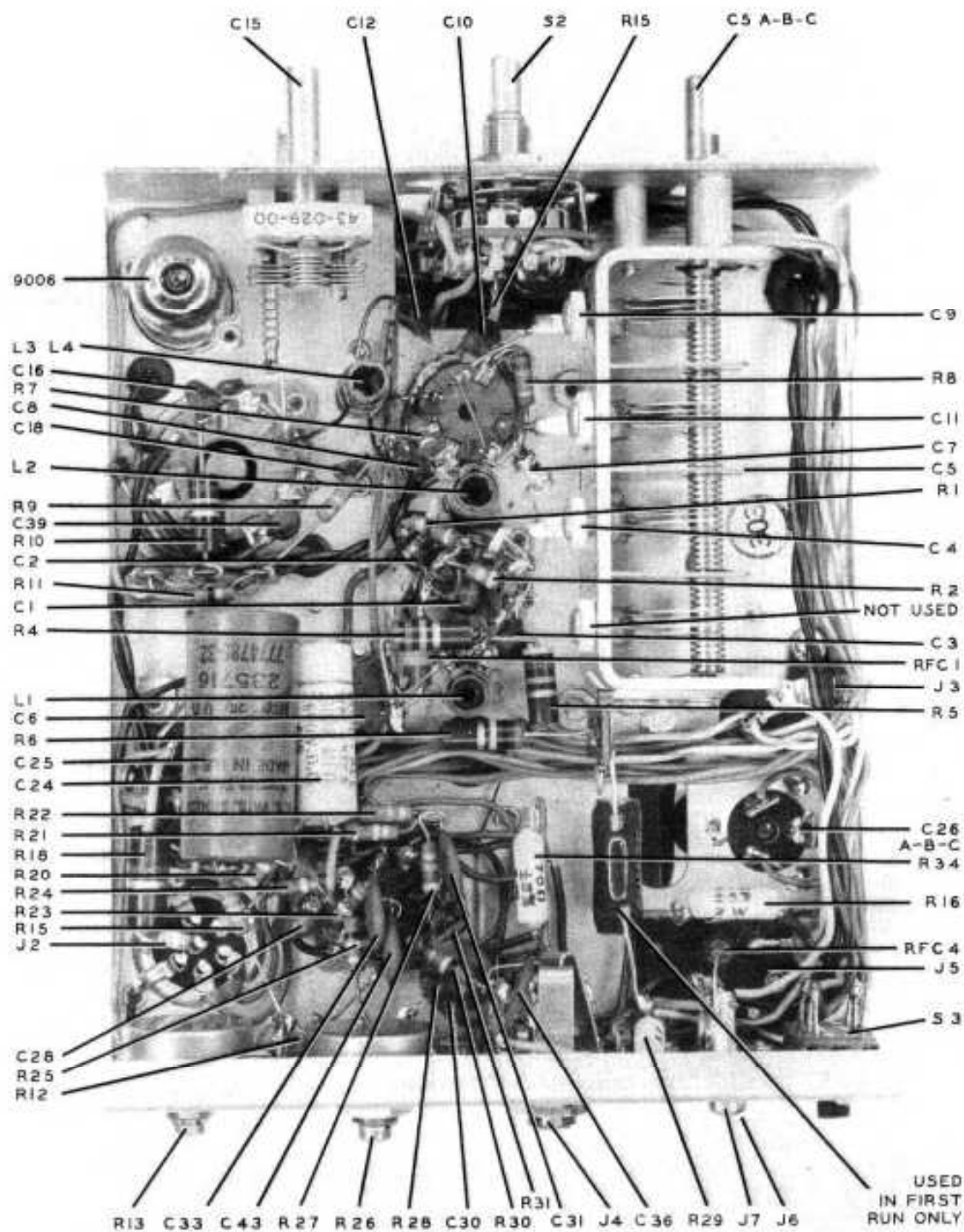
6 METER TRANSMITTER — BOTTOM VIEW
