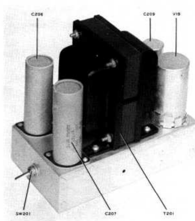
POWER SUPPLY — TOP VIEW
