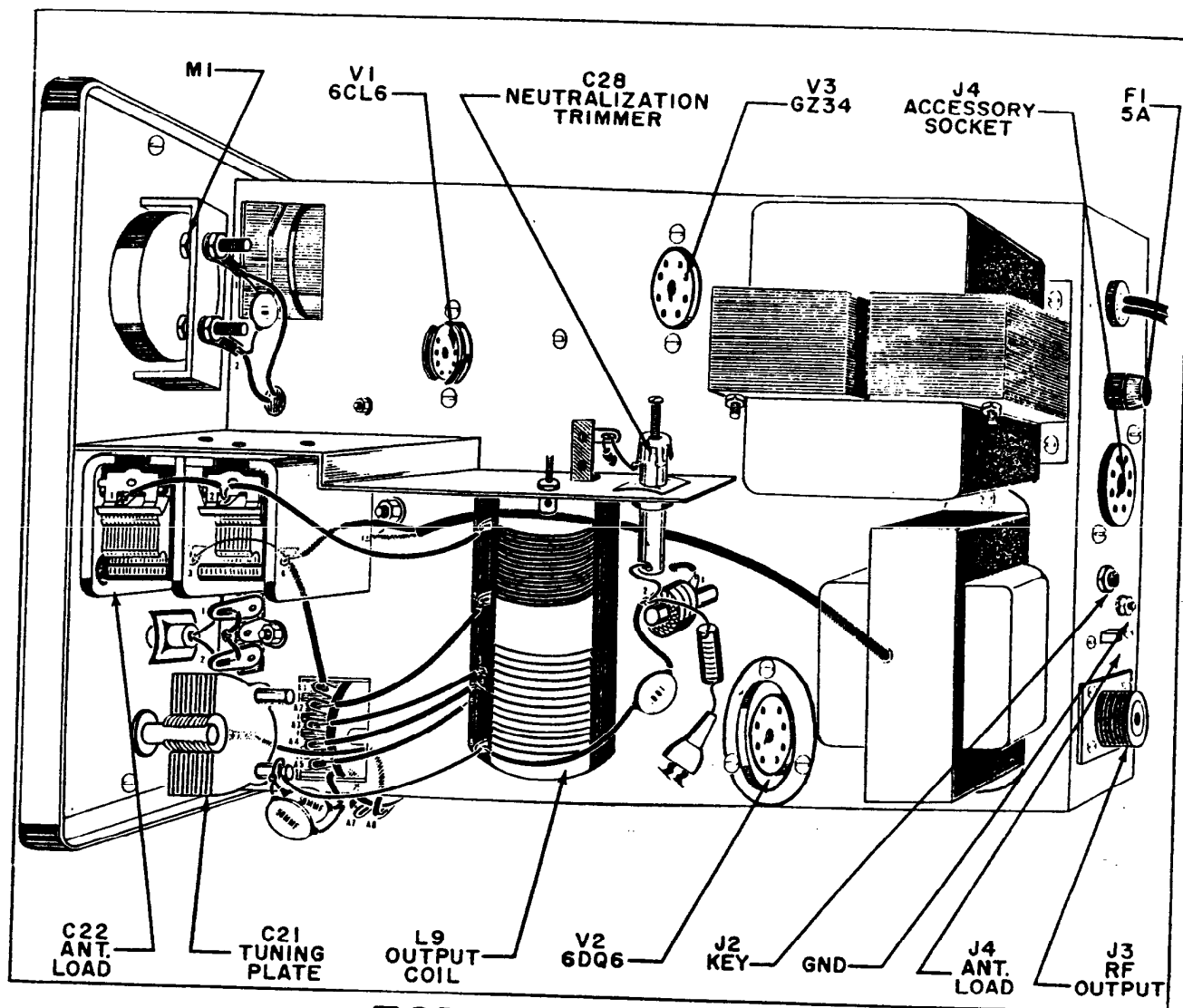
TOP VIEW FIGURE 4
