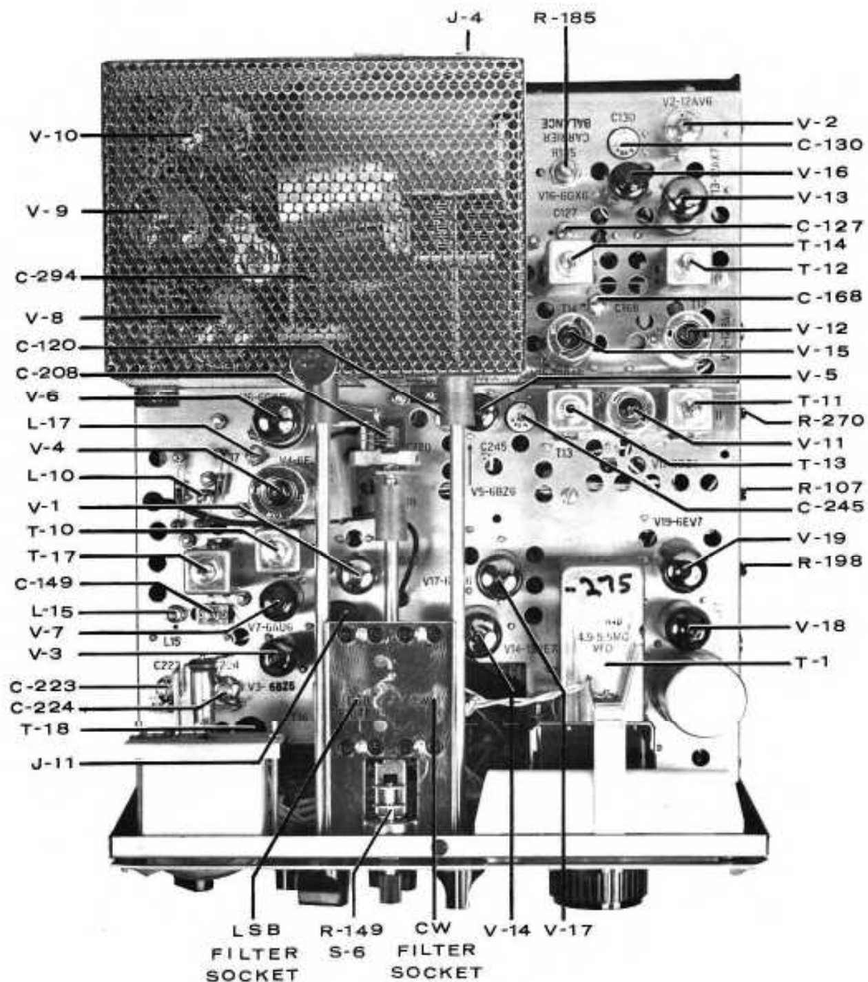
FIG.14 — TOP VIEW
