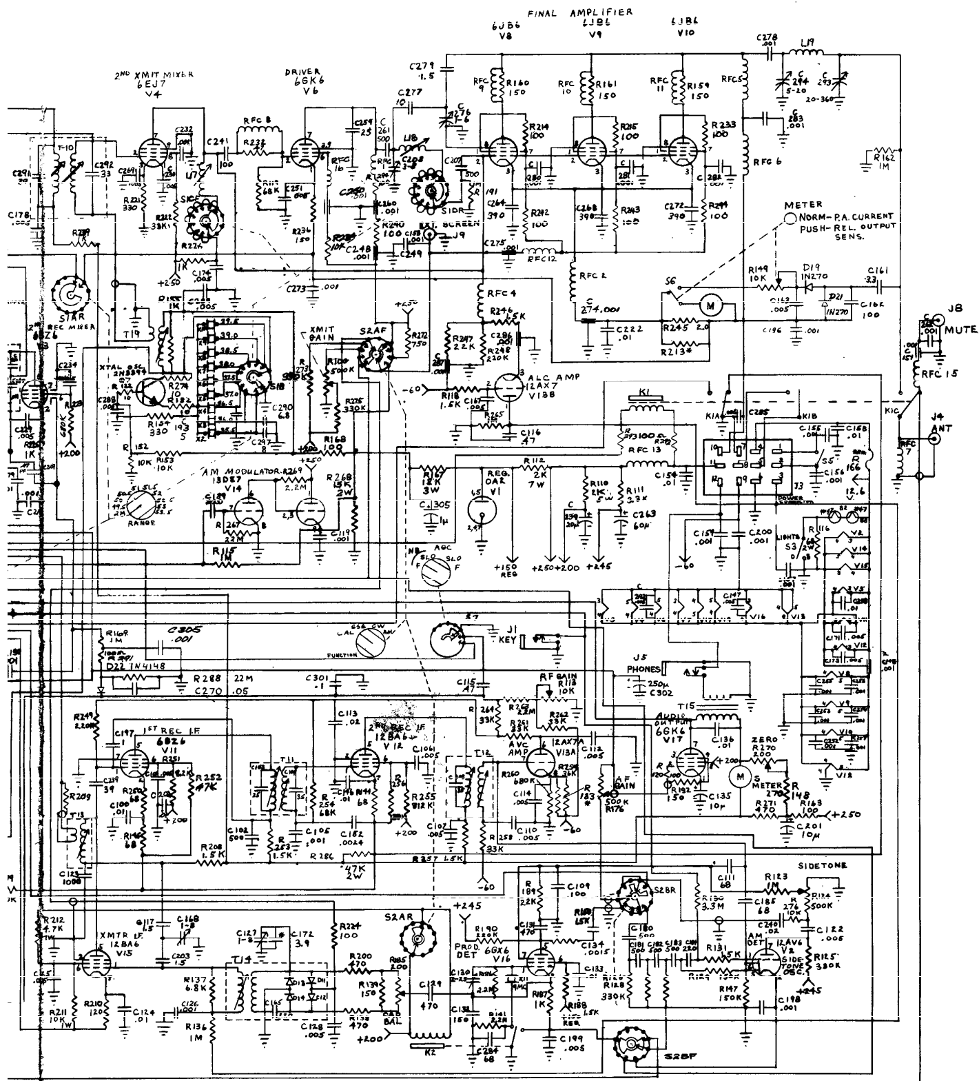
16 SCHEMATIC DIAGRAM MODEL TR-6 TRANSCEIVER 01-170
