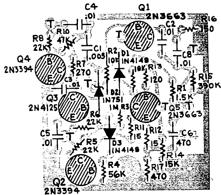
TA-4 CIRCUIT BOARD
