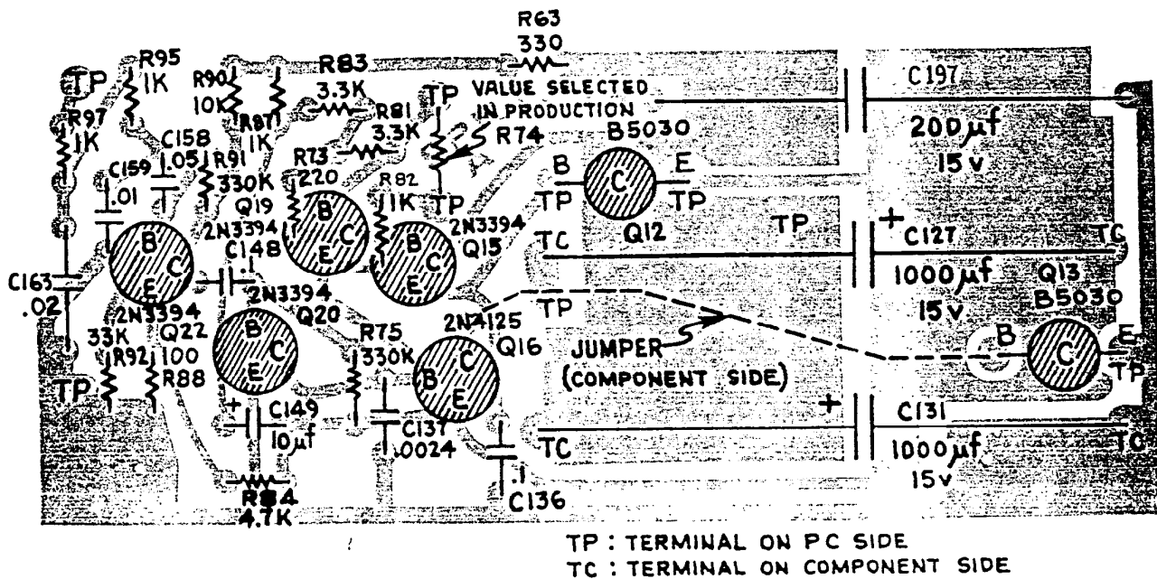
AUDIO AMPLIFIER CIRCUIT BOARD Figure 37
