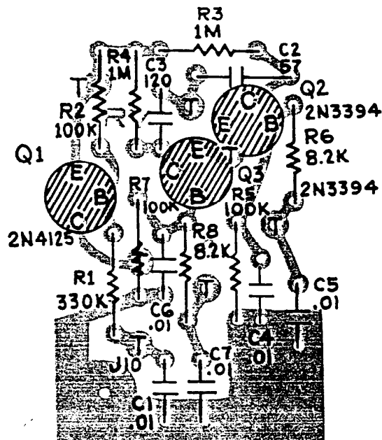
RY-4 CIRCUIT BOARD
