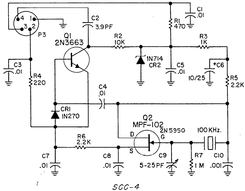
SCC-4 SCHEMATIC DIAGRAM
