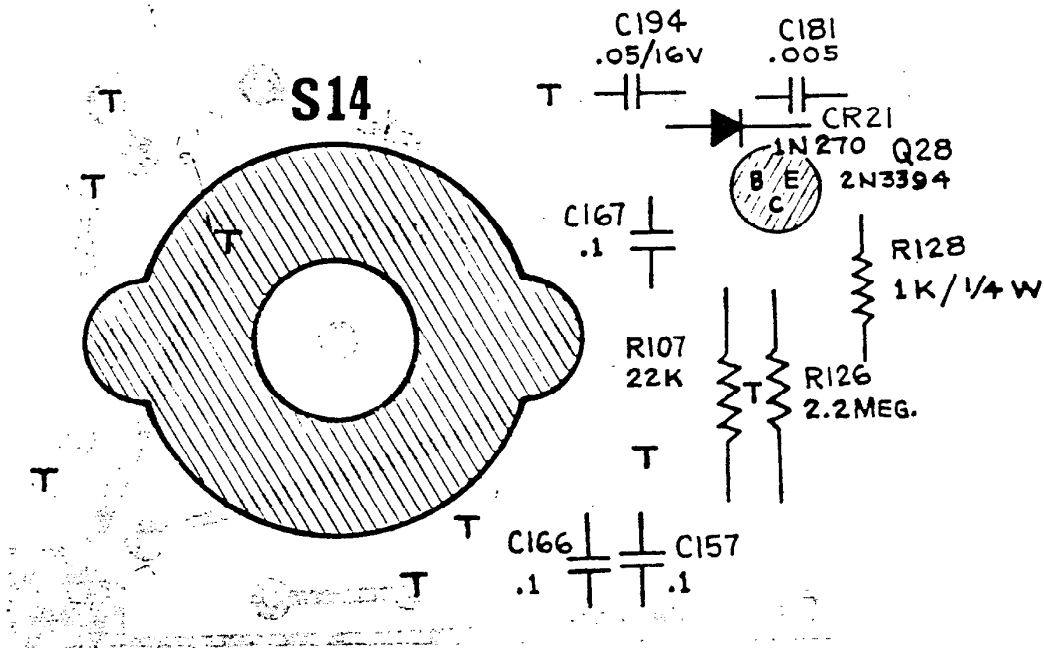
AM DETECTOR CIRCUIT BOARD Figure 36
