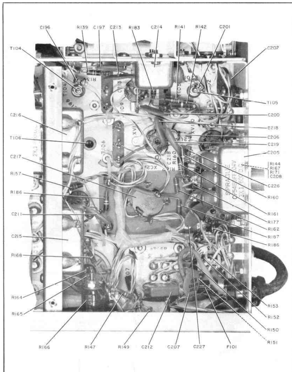
Figure 7-5. 51J-4 Bottom View, Compartment 2
